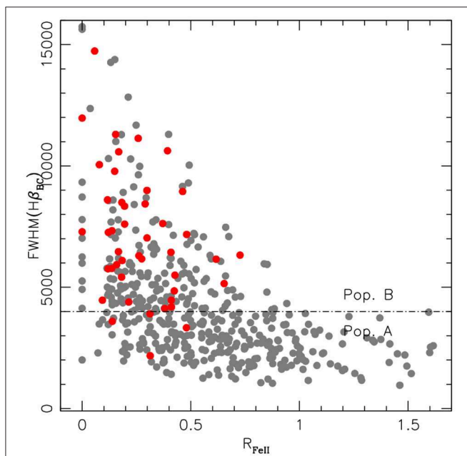
FIGURE 6 | The 4DE1 optical plane involving the width of H\beta and the strength of optical FeII. The horizontal line marks the boundary between population A (lower half of the diagram) and B (upper half) sources. Source occupation is shown for the 470 brightest SDSS-DR5 quasars ( z < 0.75 ) with highest S/N SDSS spectra (Zamfir et al., 2008). Gray and red dots represent RQ and lobe dominated LD RL quasars. The latter class shows a strong preference for the Population B zone.
