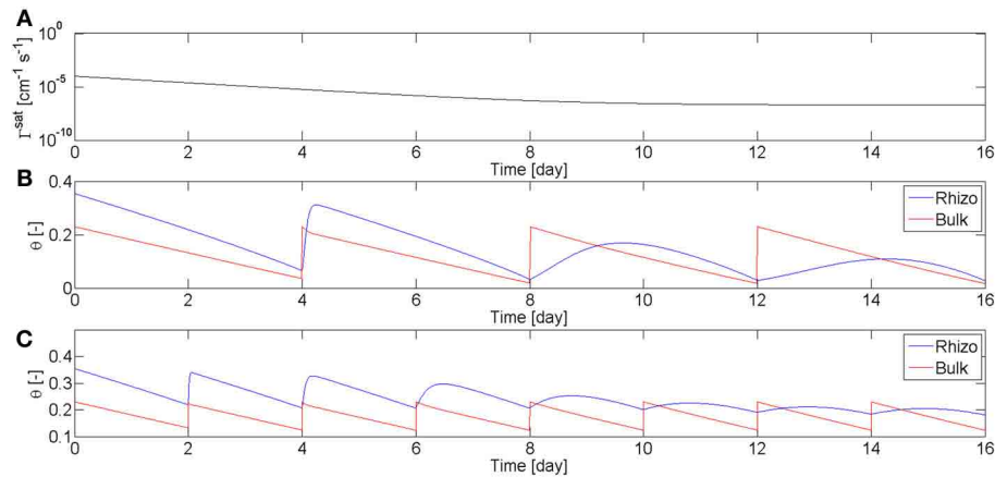
FIGURE 6 | Water content in rhizosphere (blue) and bulk soil (red) during drying and wetting cycles simulated using the model in Equation (2–5).
