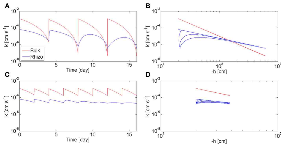
FIGURE 7 | Hydraulic conductivity of bulk soil k_b and rhizosphere k_{rh} during varying drying/wetting as predicted by the model. (A) k_b and k_{rh} as a function of time during the 4 days drying cycles of Figure 6B . When the soil was wet, k_b > k_{rh} . As the soil became dry, the two curves crossed each other and k_b < k_{rh} . As the number of drying/wetting cycles increased, the
