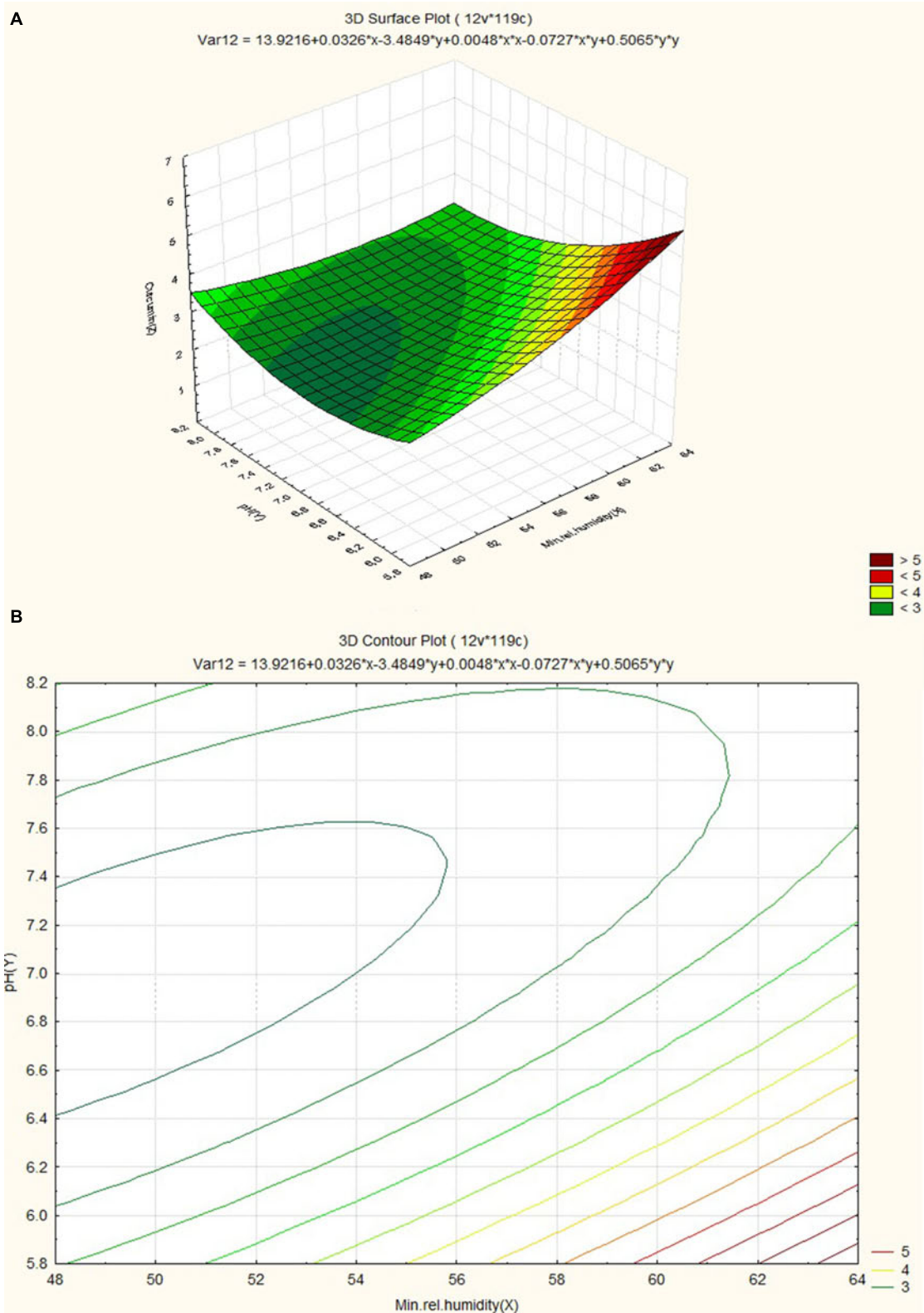
FIGURE 8 | (A) Surface plot for combined effect of pH and minimum relative humidity on curcumin content. (B) Contour plot for combined effect of pH and minimum relative humidity on curcumin content.
