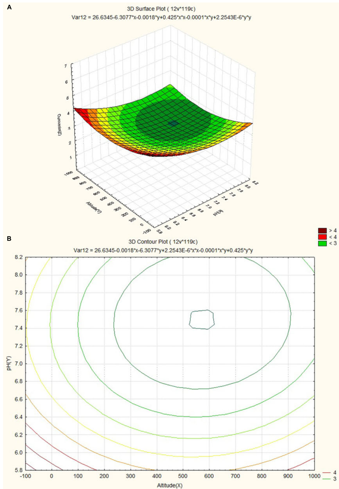
FIGURE 7 | (A) Surface plots for combined effect of altitude and pH on curcumin content. (B) Contour plots for combined effect of altitude and pH on curcumin content.
