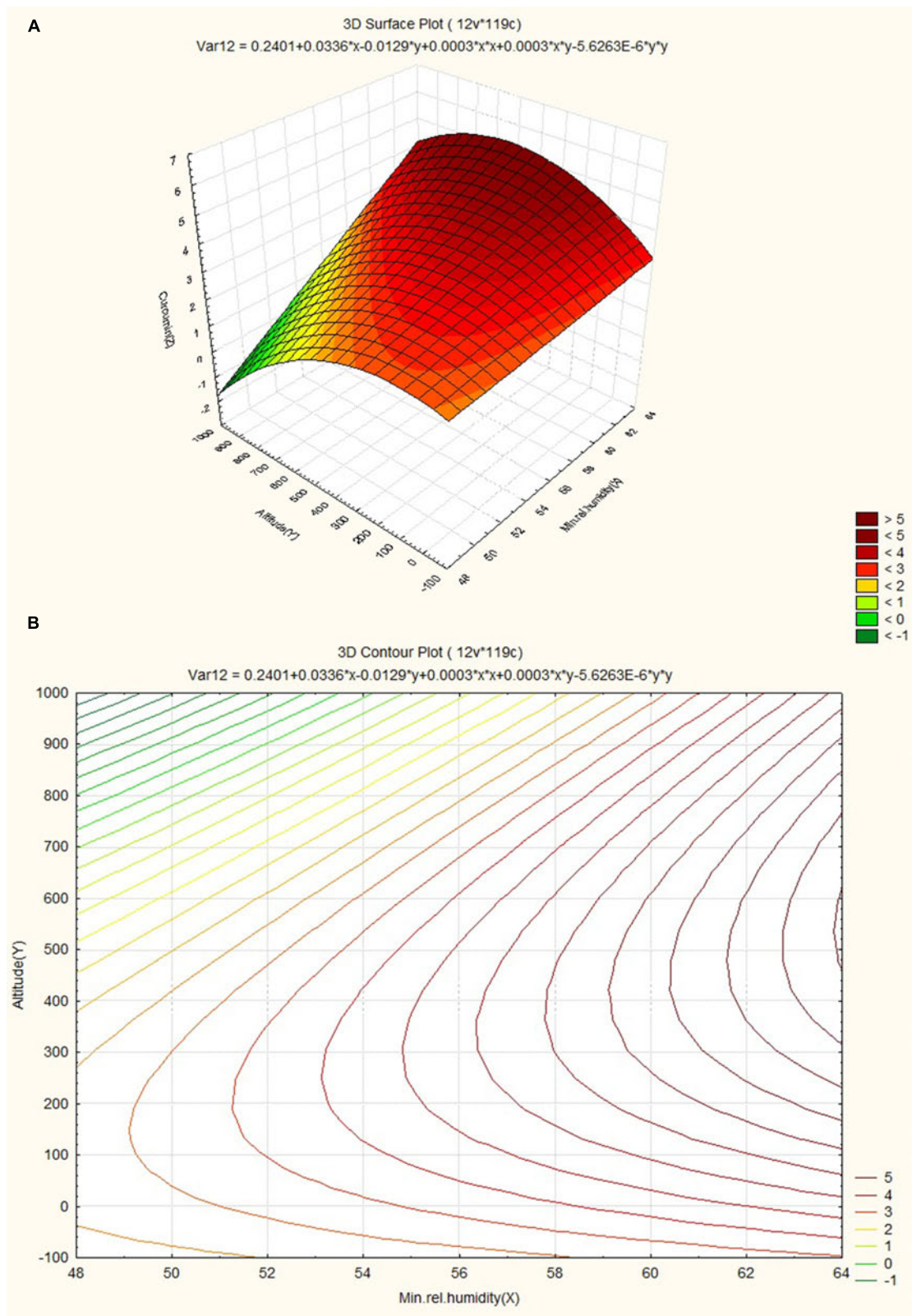
FIGURE 4 | (A) Surface plot for combined effect of altitude and minimum relative humidity on curcumin content. (B) Contour plot for combined effect of altitude and minimum relative humidity on curcumin content.
