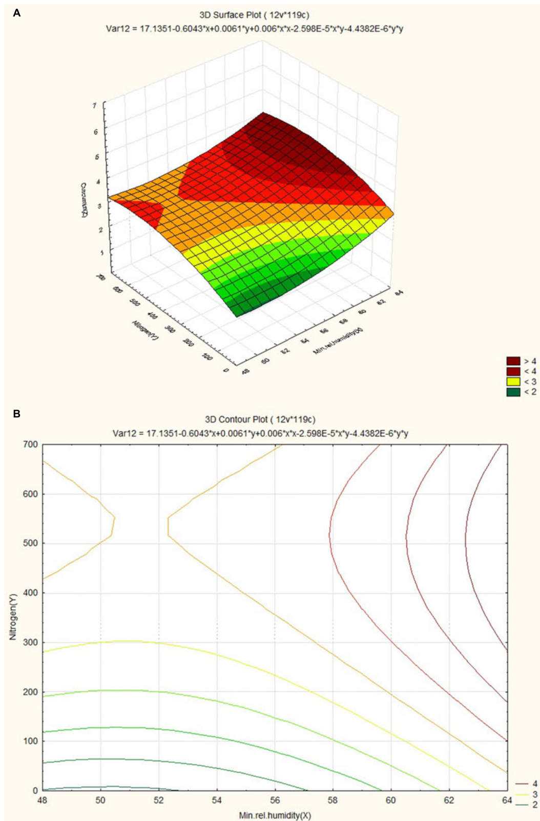
FIGURE 6 | (A) Surface plots for combined effect of nitrogen and minimum relative humidity on curcumin content. (B) Contour plot for combined effect of nitrogen and minimum relative humidity on curcumin content.
