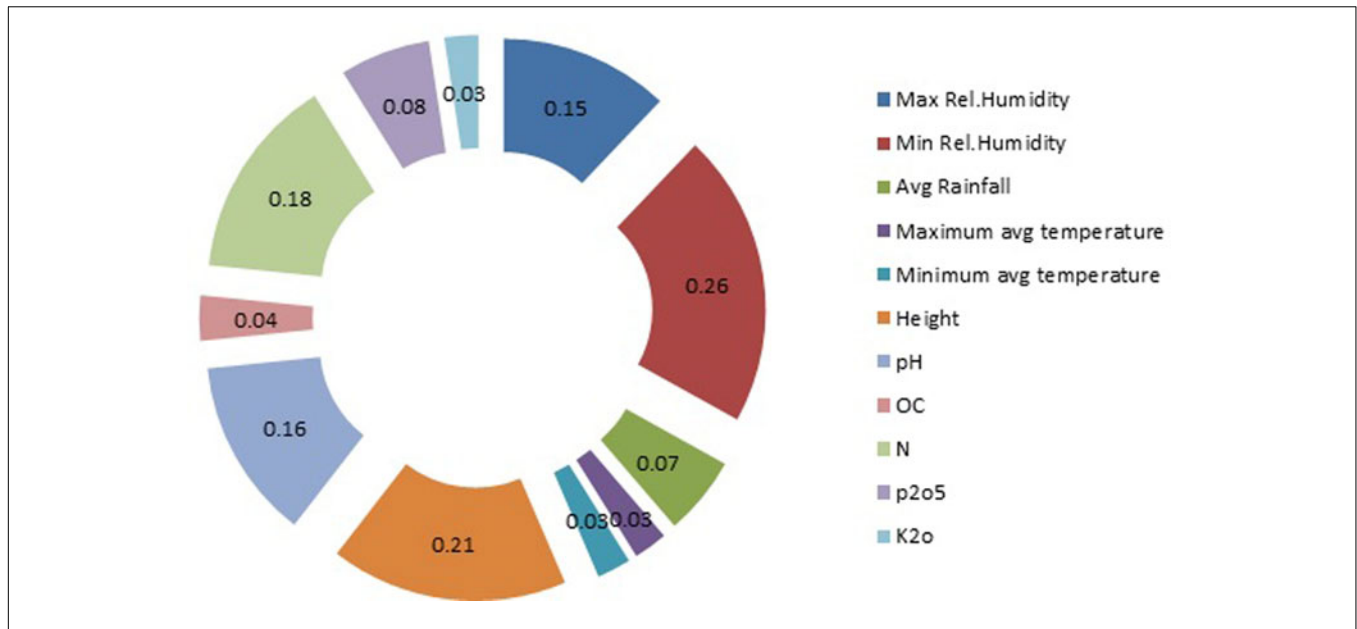
FIGURE 10 | Sensitivity analysis of input parameters on curcumin yield (output).
