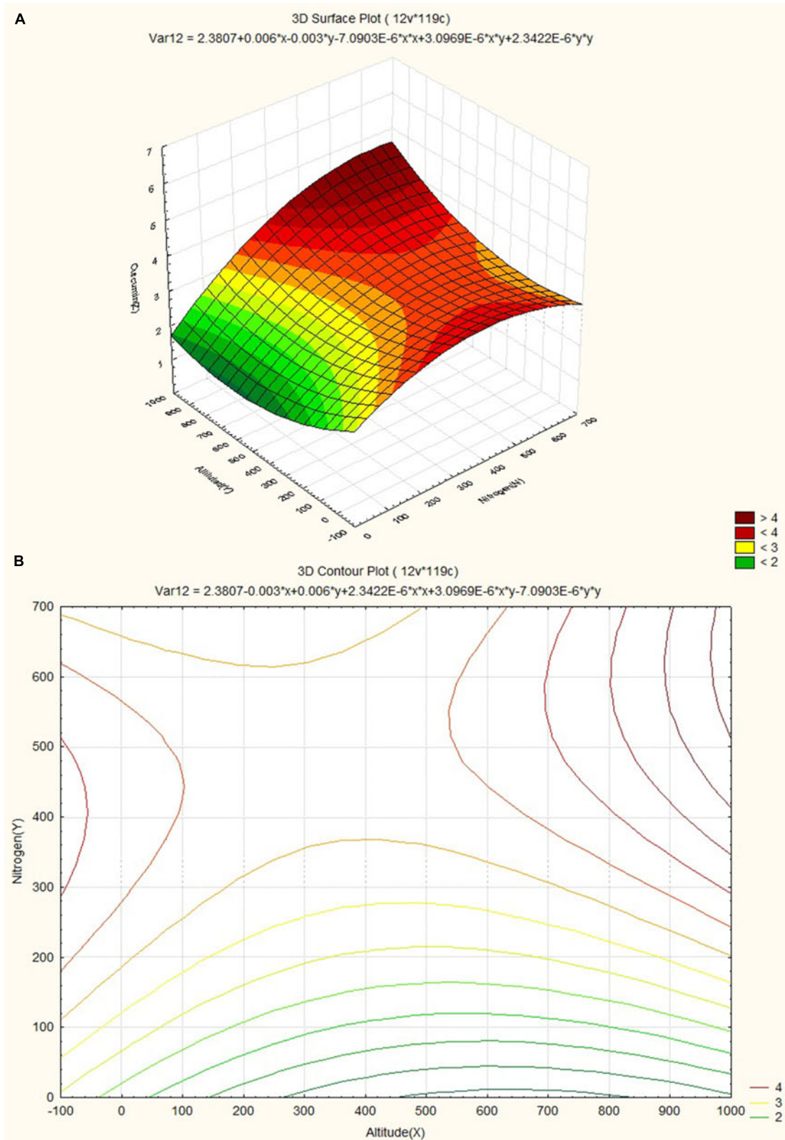
FIGURE 5 | (A) Surface plot for combined effect of altitude and soil nitrogen content on curcumin content. (B) Contour plot for combined effect of altitude and soil nitrogen content on curcumin content.
