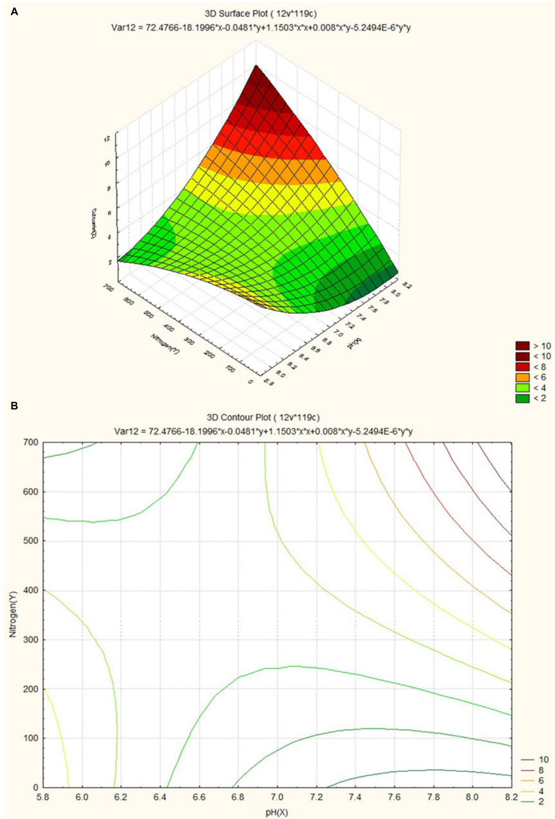
FIGURE 9 | (A) Surface plot for combined effect of nitrogen and pH on curcumin content. (B) Contour plot for combined effect of nitrogen and pH on curcumin content.
