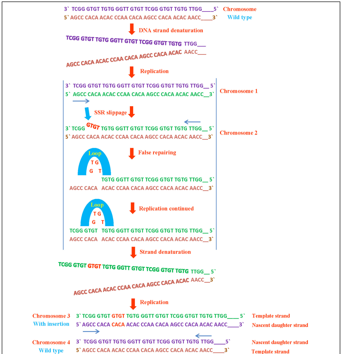
FIGURE 3 | SSR insertion during DNA replication. If a SSR slips or loops out backward from template strand, it rearranges and inserted in form of duplication or at other site in template strand which mutates the normal sequence leading to the translational and translational mutations.
