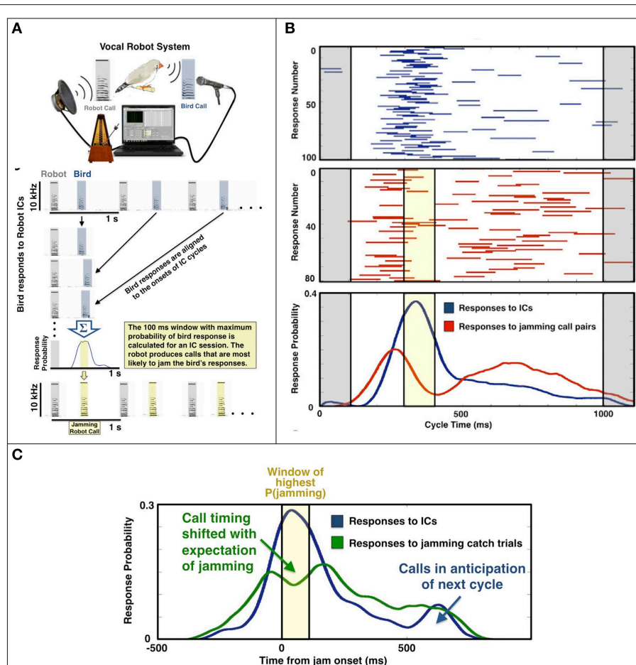
FIGURE 2 | Vocal Robot and jamming avoidance (From Benichov et al., 2016). (A) A bird interacts with isochronous calls (ICs) generated by a vocal robot at rate of 1 Hz. The bird's stereotyped response latencies are used to determine a window of maximum jamming probability (yellow). (B) A bird's responses (blue) across 1000 ms robot IC cycles (gray) and responses (red) across a subsequent session containing jamming robot calls (yellow). The bird shifts its response probability distribution to avoid jamming. (C) Cumulative response distributions across 12 birds, aligned to their window of maximum jamming probability (yellow), for ICs (blue), and for jamming catch trials (green) that contain only a single robot call.
