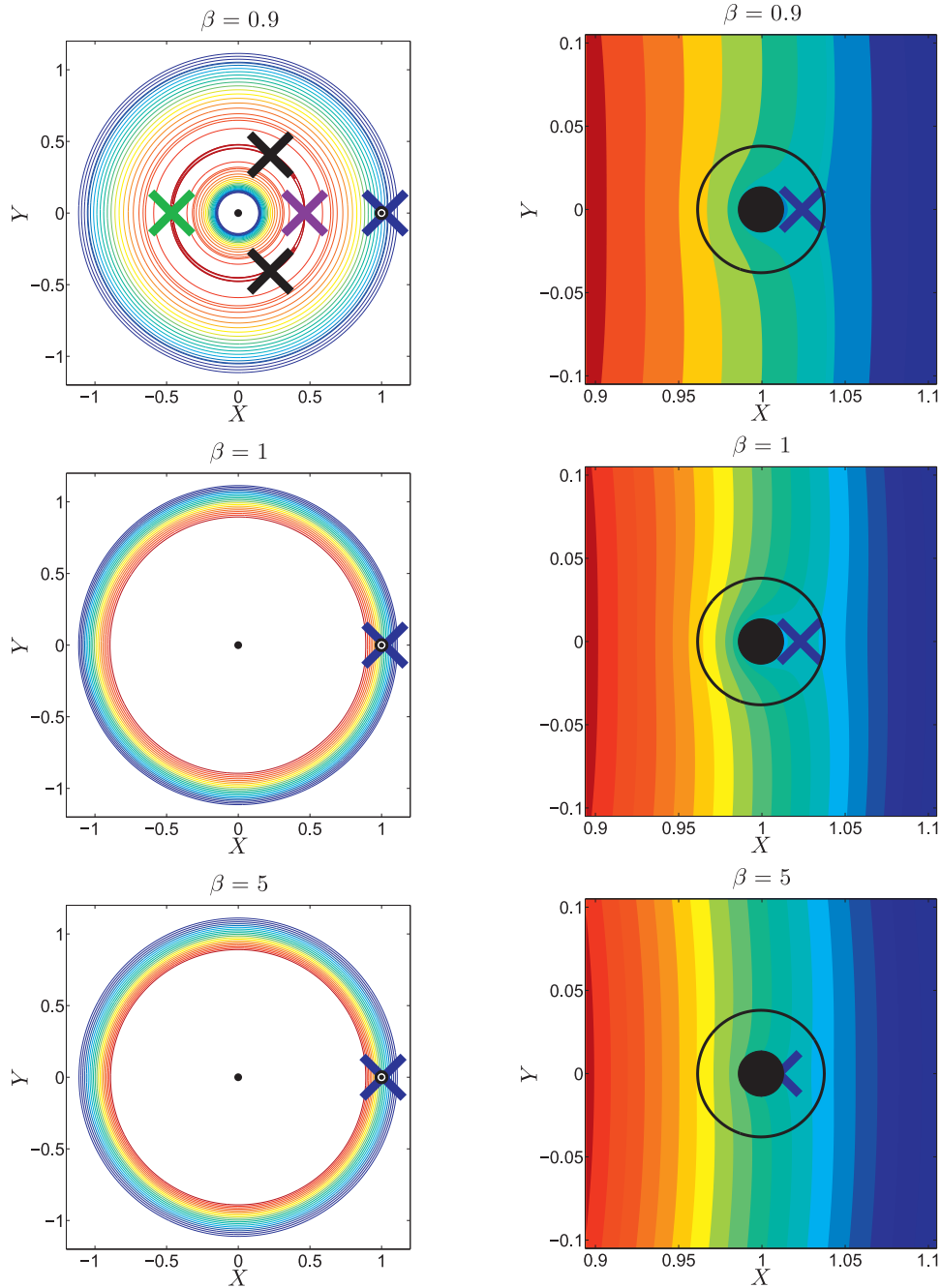
Fig. 3. Same as Fig. 2 for \beta = 0.9, 1 and 5 for HD 209458b.
