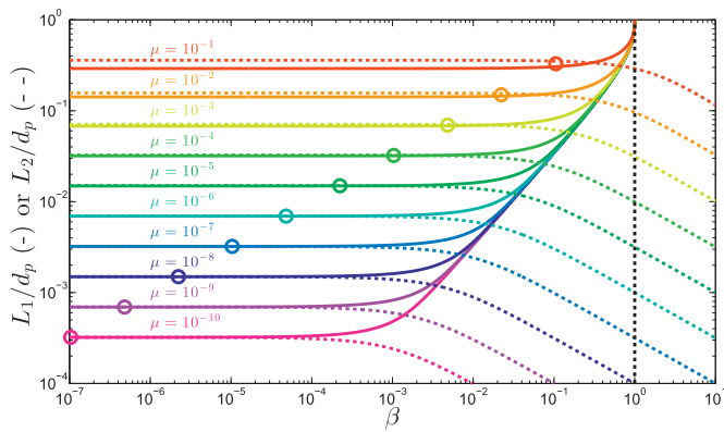
Fig. 6. Relative distances of L_1 and L_2 in planet-star distance ( d_p ) for different values of \mu . The solid lines correspond to the L_1 position for a given \mu and the dashed lines to L_2 . The circles correspond to the \beta_c(\mu) value for which the L_1 and L_2 have the same potential: for \beta > \beta_c(\mu) as defined by the circle, this is easier for a particle to escape through L_2 than L_1 . The horizontal line at \beta = 1 is the limit from which L_1 does not exist any more.
