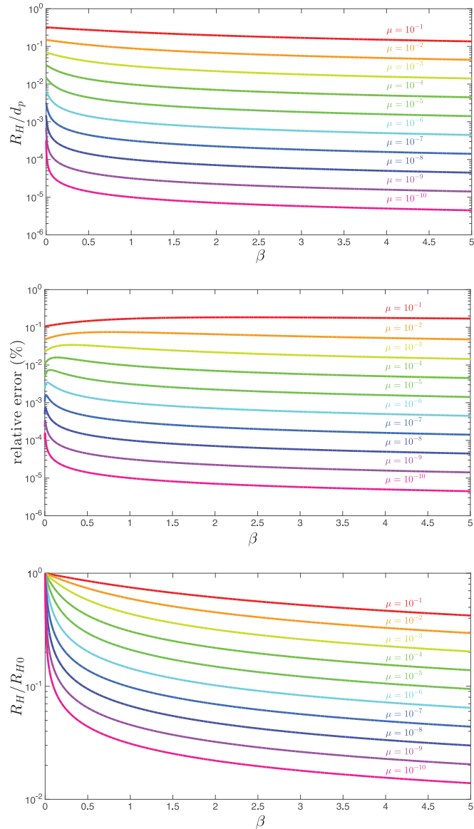
Fig. 4. (Upper panel) Ratio between the generalized Hill sphere radius and the planet-star distance as a function of \beta . (Middle panel) Relative difference between the exact numerical root from Eq. (2) and our analytical solution from Eq. (3). (Lower panel) Same as upper panel, with the modified Hill sphere radius scaled with the Hill sphere radius for \beta = 0 (pure CR3BP), for different \mu values. For \beta = 0 , we have the usual value of the Hill sphere radius \sqrt[3]{\mu/3} without radiation pressure. For higher \beta , the modified Hill sphere radius converges asymptotically to \sqrt{\mu/\beta} , i.e. the exopause distance discussed by Beth et al. (2016b).
