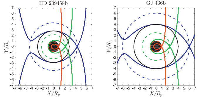
Fig. 5. Equipotentials around HD 209458b (left) and GJ 436b (right) for different radiation pressure intensities: \beta = 0 (blue), 0.6 (green; nominal case for GJ 436b) and 4 (red; nominal case for HD 209458b). The corresponding Hill sphere is the circle in dotted line with the corresponding color. The filled centered circle corresponds to the solid core of the planet and the black solid circle to the circle bordered by the Roche lobe often assimilated to the top of the dense atmosphere or to the exobase. (For interpretation of the references to color in this figure legend, the reader is referred to the web version of this article.)
