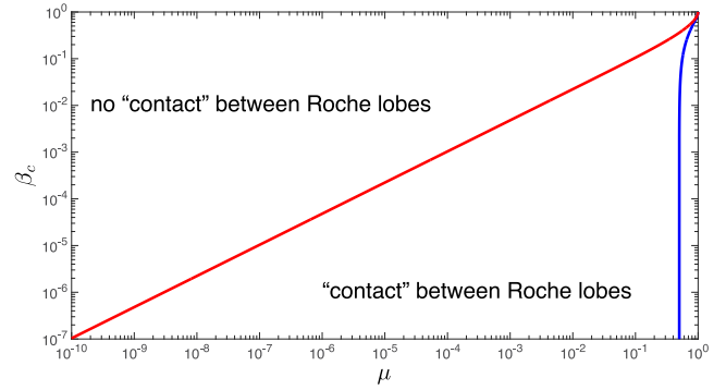
Fig. 1. Plots of critical \beta values adapted from Schuerman (1972) in log-scale, more adapted for our approach. The red curve represents the \beta_c value for which L_1 and L_2 share the same energy and thus the same equipotential. The blue plot is similar but applied between L_1 and L_3 and can exist only for \mu > 0.5 (this does not make sense for us because this means that the planet is heavier than the star). We retrieve the asymptotic behavior derived by Schuerman (1972) for \mu = o(1) : \beta_c \sim (\mu/3)^{2/3} . (For interpretation of the references to color in this figure legend, the reader is referred to the web version of this article.)
