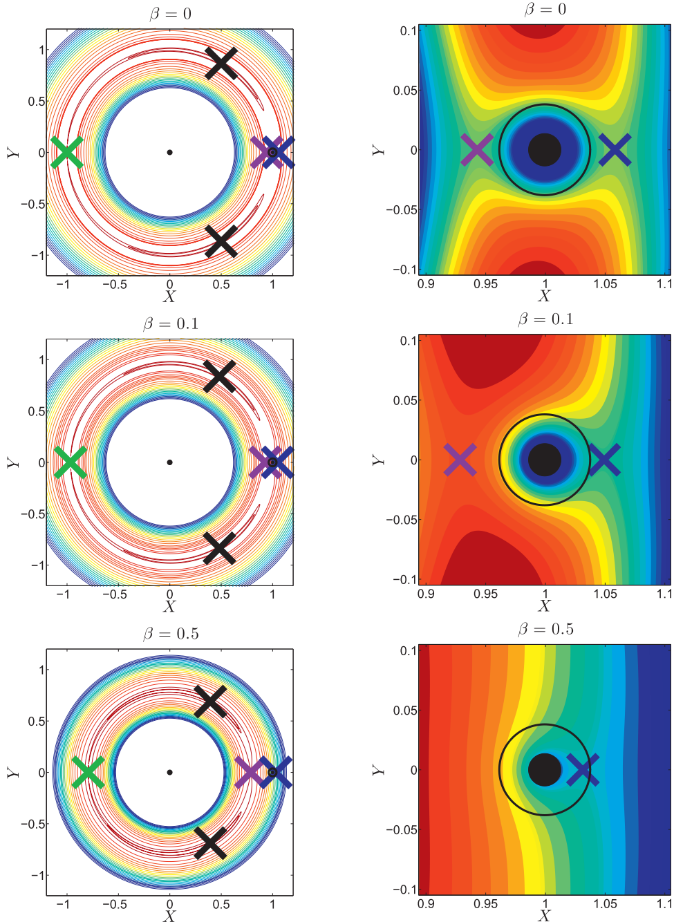
Fig. 2. Levels of effective potential \Omega for \beta = 0 (pure CR3BP, upper panels), 0.1 and 0.5 for HD 209458b. The left panels provide a global picture of the equipotentials in the system and the right ones correspond to a zoom in the vicinity of HD 209458b. Warm/cold colors refer to high/low potential energies. The crosses define the Lagrange points: L_1 (violet), L_2 (blue), L_3 (green), L_4 and L_5 (black). The central point corresponds to the star position. The black point around (1 - \mu, 0) corresponds to the true planetary size and the surrounding black circle to the exobase with its supposed size. (For interpretation of the references to color in this figure legend, the reader is referred to the web version of this article.)
