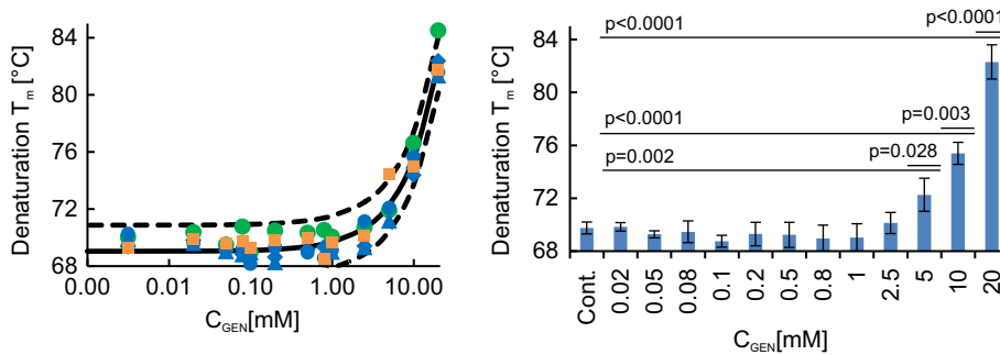
Fig. 6. (Left) denaturation temperatures as measured by DSC. Fit: linear model ( t_m = 0.66 \text{ }^\circ\text{C}/\text{mM} \times [\text{GEN}] \text{ mM} + 69.26 \text{ }^\circ\text{C} , R^2 = 0.96 ) with \log_{10} transformed concentrations and 95% confidence intervals. 0 mM GEN is plotted at 0.003 mM. \blacksquare 24 h GEN treatment, \blacklozenge 72 h GEN treatment, \bullet 144 h GEN treatment. (Right) Bars indicate significant differences from post hoc pairwise comparison with a significant main effect. Only significant differences between adjacent groups or to controls were plotted as all other pairwise comparisons were significantly different, except below a concentration of 2.5 mM, for which there was no effect. Markers of the same color but different shape ( \blacksquare , \blacklozenge and \bullet ) indicate samples from the same experimental condition but from different horses.
