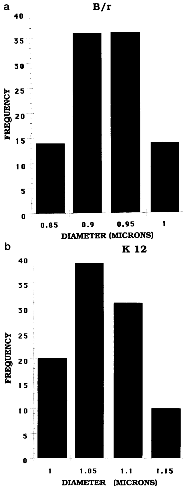
FIGURE 6 Histograms showing distribution of diameters of individual cells assumed to obtain fit of Fig. 5, (a) for E. coli B/r, and (b) for E. coli K12
