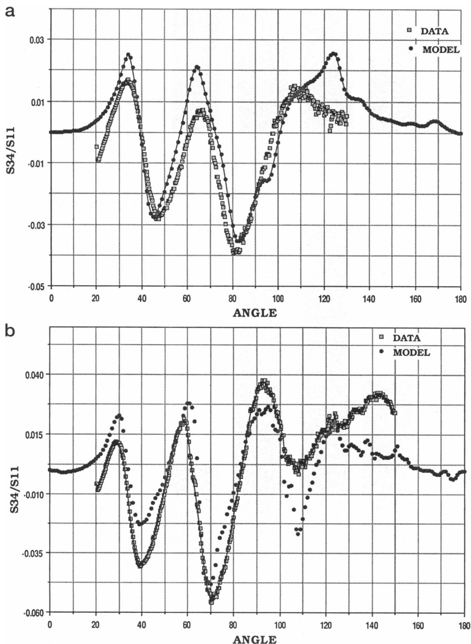
FIGURE 5 (a) S_{34}/S_{11} versus angle for experimental data from log-phase E. coli B/r. ( \square ) Data; ( \bullet ) Model. (b) Same for E. coli K12. Scattering wavelength is 502.6 nm.
