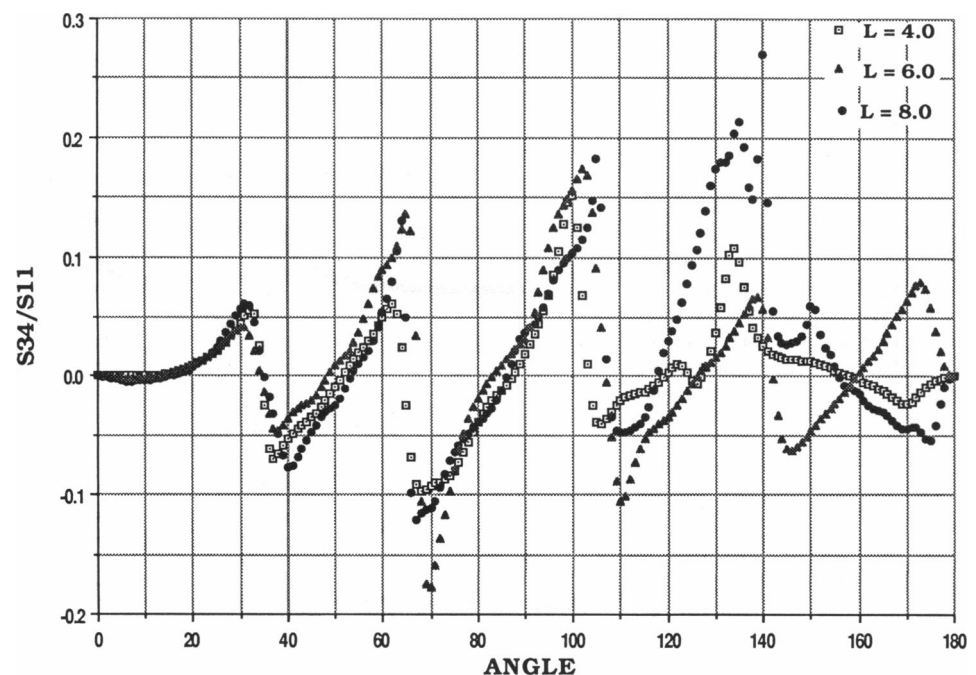
FIGURE 4 Rotationally averaged graph of S_{34}/S_{11} for single-sized capped cylindrical bacteria of lengths 4.0 , 6.0 , and 8.0 \mu\text{m} but all of diameter 1.34 \mu\text{m} calculated with the CDM. Scattering wavelength is 633 \text{ nm} .
