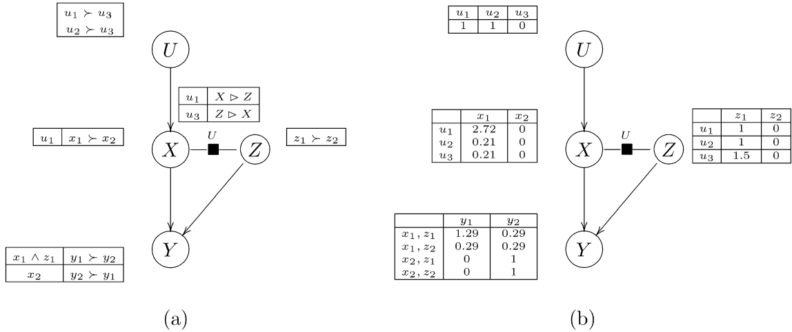
Fig. 7. (a) Acyclic TCP-net with a ci-arc for Example 2; (b) The value function generated for that TCP-net.
