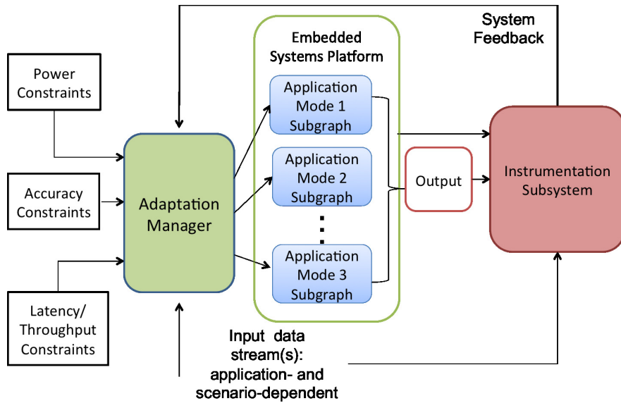
Figure 1: Data-driven, multi-mode embedded system design flow.
