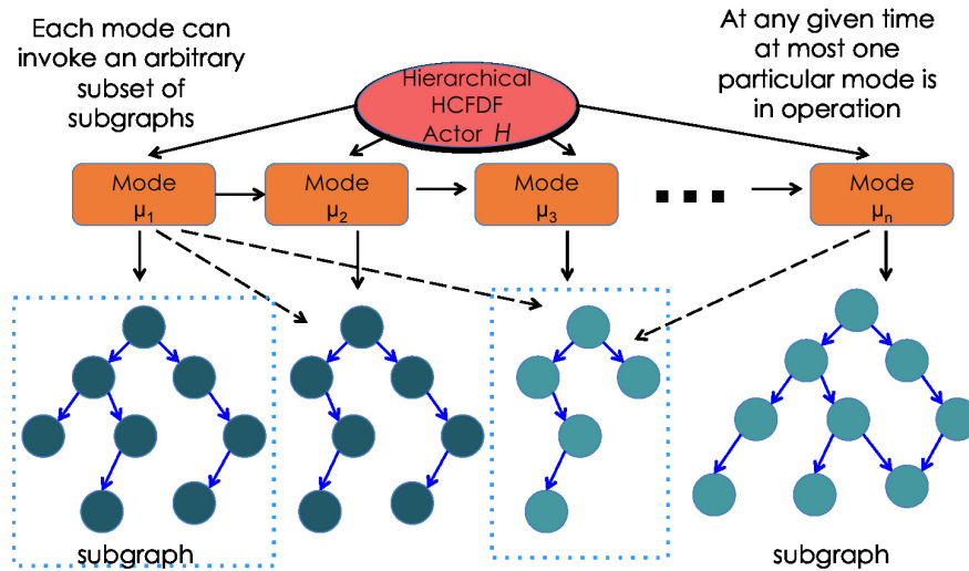
Figure 2: Modeling multi-mode DDDAS designs using HCFDF graphs.
