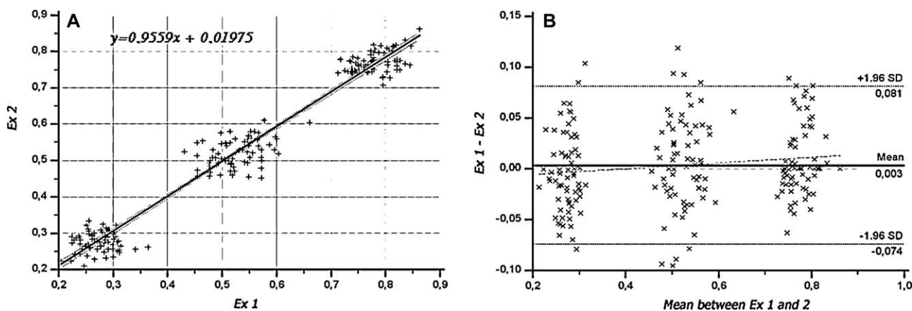
Figure 6 Interobserver reproducibility. A: regression line showing excellent correlation between examiner 2 and examiner 1. B: Bland-Altman plots showing dispersion of measurement differences between examiner 2 and examiner 1.
