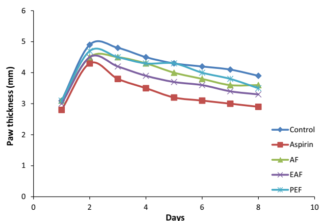
Figure 1 The paw thickness of various fractions of MELSB. EAF exhibits time-dependent anti-inflammatory effects in a similar fashion to that of aspirin.
