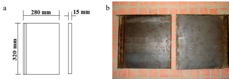
Fig. 4 (a) Tile Specimen dimensions,(b)Tile Moulds with cover
