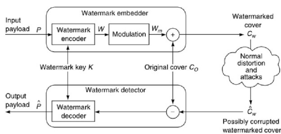
Figure 1. Nonblind watermarking framework
