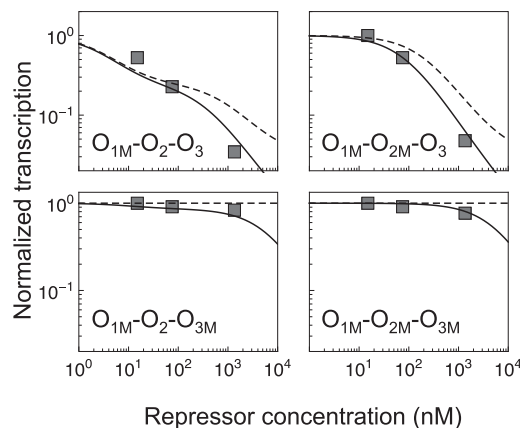
FIGURE 5 Complete deletions versus weak binding. The normalized transcription ( \bar{I}/I_{\max} ) for the four configurations with O_{1M} is shown for the model as in Fig. 4 A (solid line); for the model assuming that the free energy of binding to O_{1M} is infinite, as in a complete deletion (dashed line); and for the experimental data from Oehler et al. (14) (squares).
