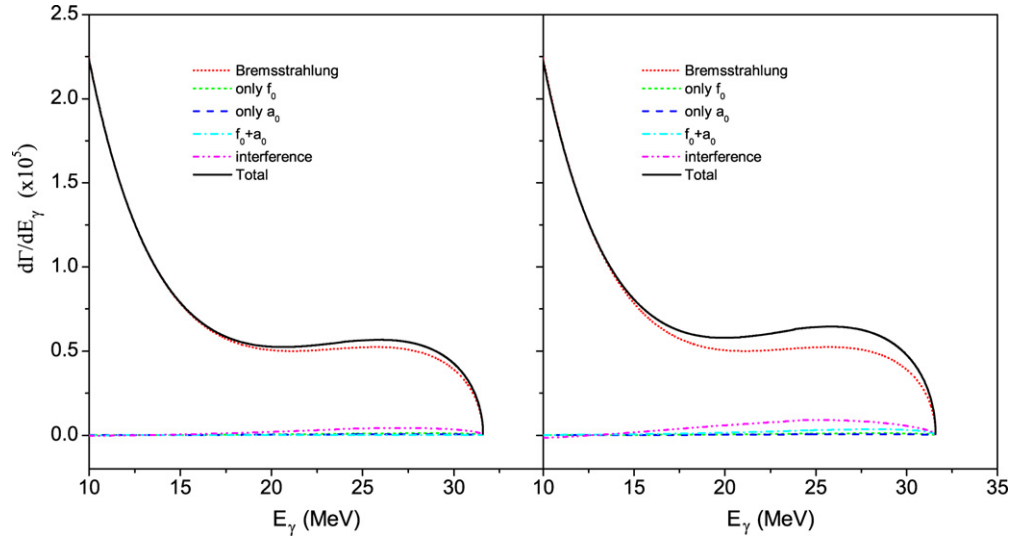
Fig. 4. The photon spectra for the decay width of \phi \rightarrow K^+K^-\gamma in the no-structure model with g_{f_0K^+K^-} > 0 , g_{a_0K^+K^-} < 0 (left) and g_{f_0K^+K^-} > 0 , g_{a_0K^+K^-} > 0 (right). The contributions of different terms are indicated.
