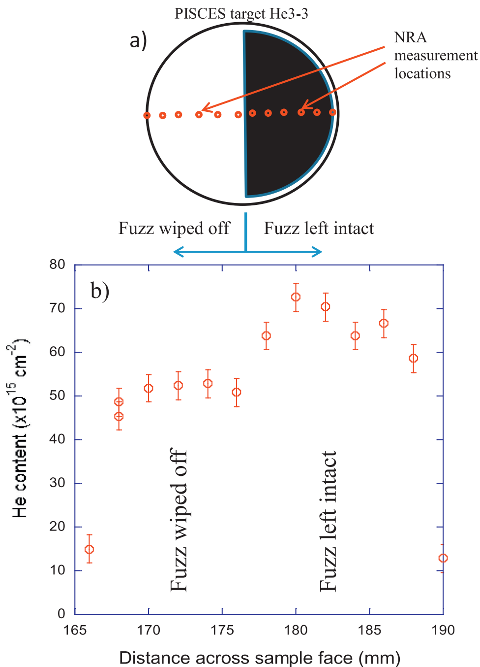
Fig. 5. Measurements were made on a fuzzy tungsten sample where (a) half the fuzz has been wiped off the surface, (b) resulting helium content in regions with and without fuzz.
