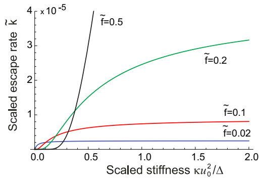
FIGURE 4 The rate of latent complex rupture (and active TGF- \beta escape), scaled in nondimensional units as \tilde{k} = k \cdot 2\sqrt{2\pi}u_0^3/9\sqrt{k_B T D} , plotted as function of substrate stiffness \kappa (also scaled in nondimensional units, see text). The curves are for different values of scaled force, \tilde{f} = Fu_0/\Delta , labeled on the plot. As the pulling force increases, the region of steepest response of the mechanosensing complex to the substrate stiffness shifts toward higher stiffness, and also becomes more diffuse—enabling a graded response, as opposed to a very sharp response at small forces on very soft substrates. To see this figure in color, go online.
