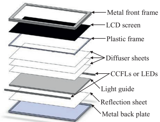
Fig. 3 Exploded view of the structural design of an LCD module (modified from McDonnel et al. [5] and Matharu et al. [12]).
