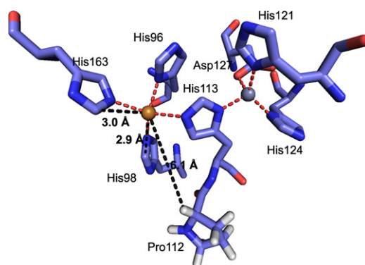
Fig. 6. Structural representation of H 2 O 2 -induced modifications of EC-SOD. The structural region of EC-SOD involved in the coordination of the copper and zinc ions is shown. The residues susceptible to oxidation (His98 and His163) and central to fragmentation (Pro112) are shown in sticks. The distances between copper and C2 of His98 and His163 and the hydrogen atom at the α-carbon of Pro112 are indicated.
