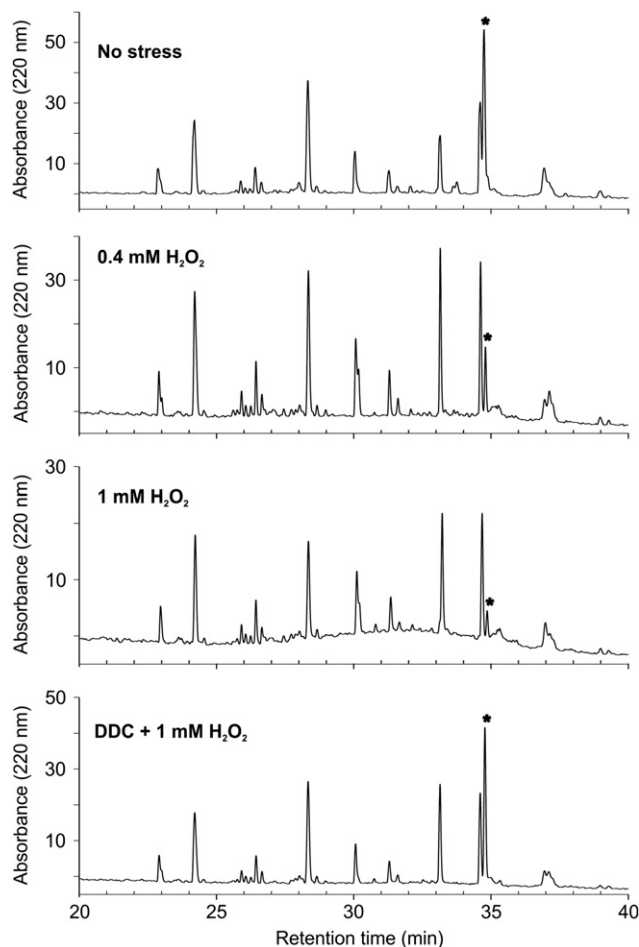
Fig. 2. Tryptic peptide maps of EC-SOD exposed to H 2 O 2 . EC-SOD and H 2 O 2 were incubated at the indicated conditions and protein subsequently digested using trypsin. The digests were separated by reverse-phase UPLC and the peptides were detected by absorbance at 220 nm. The peptide maps showed that the absorption of the S-carbamidomethylated peptide Ala94–Arg143 (*) was reduced by increasing amounts of H 2 O 2 indicating that this peptide is modified by oxidation. No significant increase in concomitant absorption could be detected in the maps. The presence of DDC inhibits the modification of the peptide showing that copper is central for the process.
