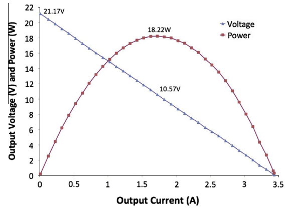
Fig. 10. Electrical characterisation of an array with three TEGs in series under mismatched temperature difference: \Delta T_{TEG\# 1} = 100 °C; \Delta T_{TEG\# 2} = 150 °C; \Delta T_{TEG\# 3} = 200 °C.
