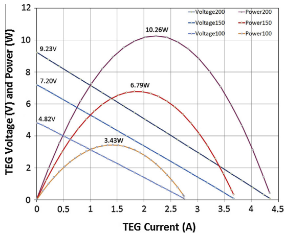
Fig. 7. Experimental electrical characterisation for the TEG module # 2. The grey dots in the curves represent experimental data points. \Delta T = 100\text{ }^\circ\text{C} , 150\text{ }^\circ\text{C} , 200\text{ }^\circ\text{C} , clamped at 2\text{ kN}/1.25\text{ MPa} .
