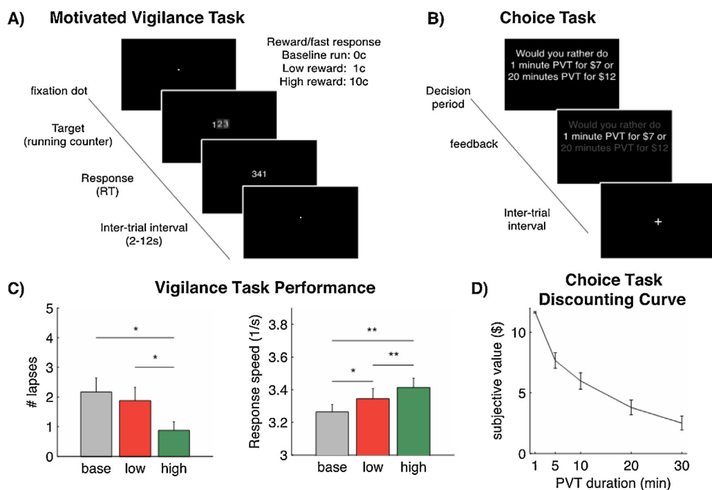
Fig. 1. Experiment 1: Schematics of a trial in (A) the Motivated Vigilance Task and (B) the Choice Task. (C) Vigilance performance under baseline, low and high reward conditions with (left) lapses of attention and (right) response speed. (D) Discounting curve in the choice task. (Error bars denote \pm 1SEM ; +p < 0.1 , *p < 0.05 , **p < 0.01 ).
