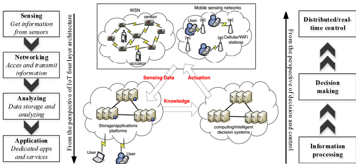
Fig. 4. CPS architecture model.
