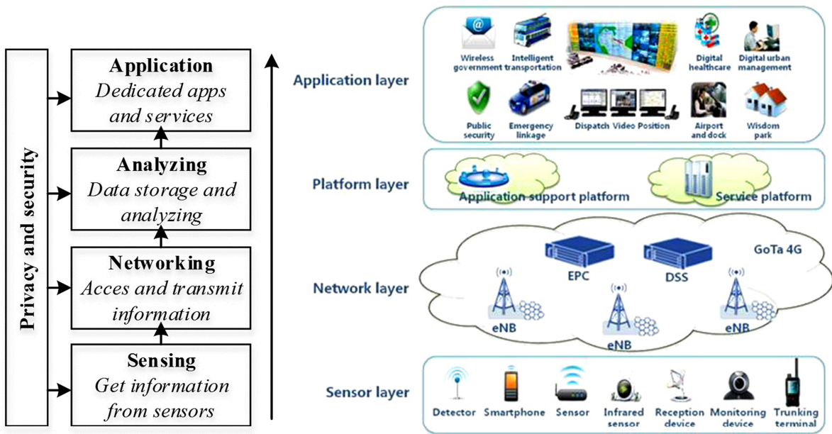
Fig. 3. Four-layer architecture of IoT, WSN, M2M and CPS.
