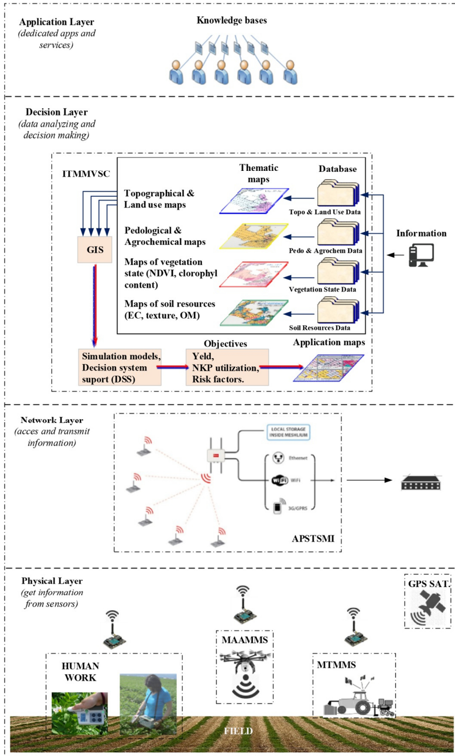
Fig. 5. CPS architecture for monitoring potato crop vegetation status.
