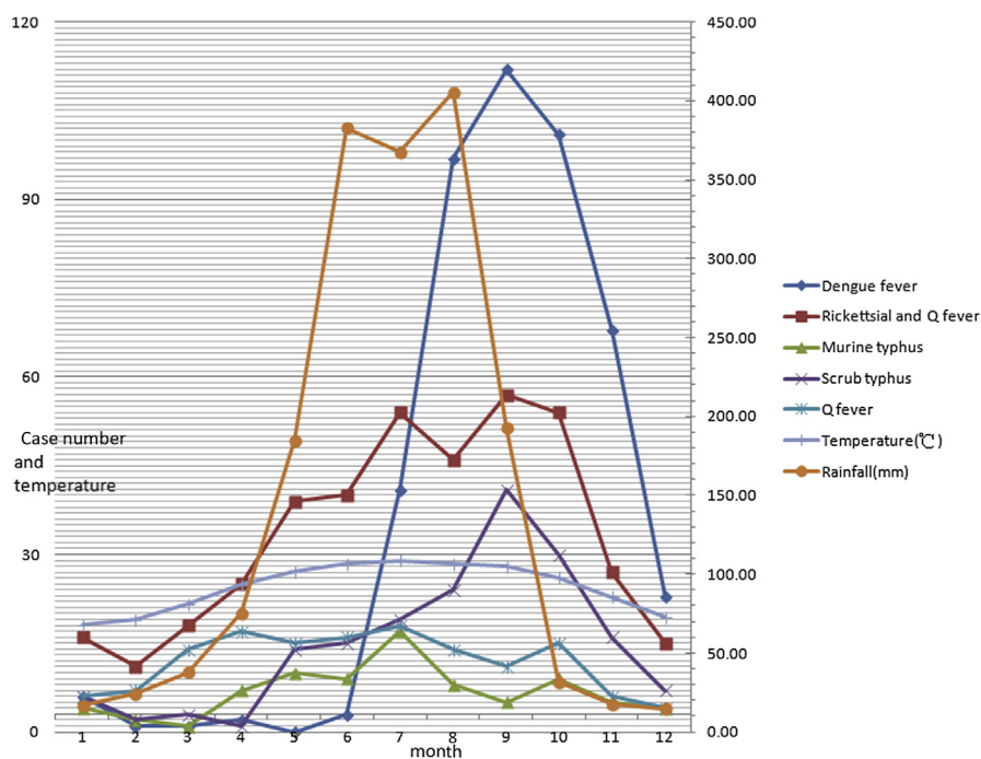
Figure 1. Monthly distribution of the 402 cases of rickettsial infection and Q fever, and the 454 cases of dengue fever (1992–2009), and their correlation with average temperature ( ^{\circ}\text{C} ) and rainfall (mm) in the Tainan and Kaohsiung areas.
