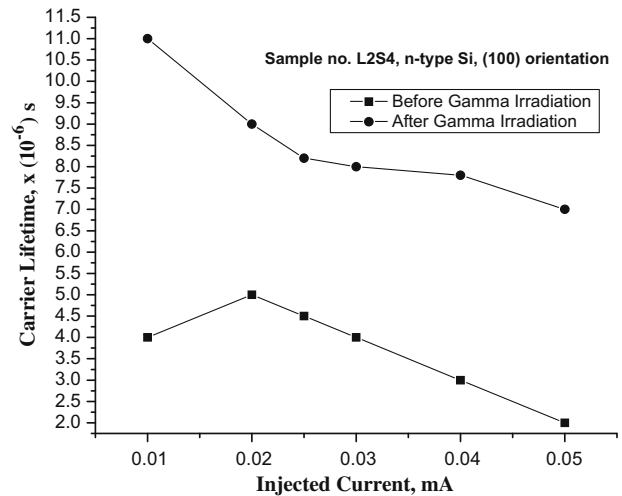
Figure 5 Carrier lifetime variation with injected current in silicon wafer.
