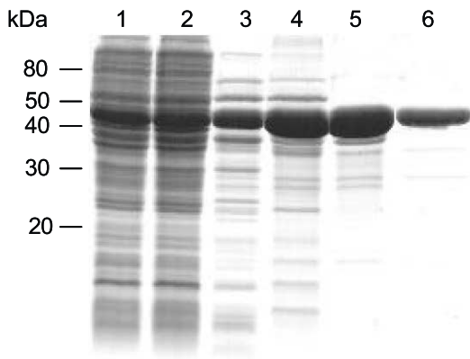
Fig. 2. Sodium dodecyl sulfate–polyacrylamide gel electrophoresis (SDS–PAGE) analysis of different fractions obtained during the purification of recombinant GcpE. 1, Crude bacterial lysate; 2, soluble proteins; 3, heat stable proteins; 4, GcpE fraction after weak anion exchange chromatography on DEAE Sepharose; 5, GcpE fraction after strong anion exchange chromatography on 15 Q Sepharose; 6, GcpE fraction after Superdex 200 gel filtration.
