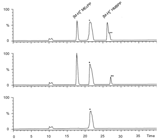
Fig. 4. HPLC-ESI-MS analysis of the GcpE reaction product. The reaction mixture containing 12 mM MEcPP, 8 mM dithionite and 20 \mu M GcpE was incubated for 1 h at 55°C (upper panel). As control, GcpE (middle panel) or MEcPP (lower panel) were omitted. Mass chromatograms were recorded for MEcPP ( m/z 277) and HMBPP ( m/z 261). As an additional major component, sulfate ( m/z 97) derived from dithionite was recorded (asterisk). An unknown compound of m/z 277 was detected as an impurity of the MEcPP sample (two asterisks).
