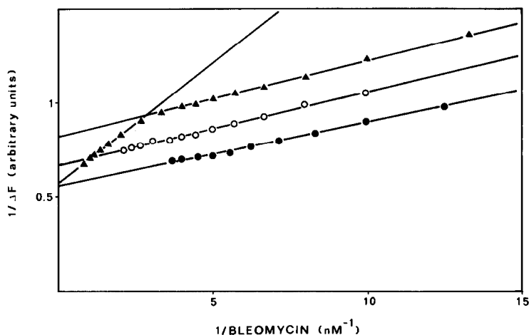
Fig.3. Lineweaver-Burk representation of the reciprocals of fluorescence decrease intensities ( \Delta F ) versus bleomycin concentrations. BLM or BLM-Fe(II) (up to 1.5 \mu\text{M} ) was added to 2 ml of Sh protein (0.4 \mu\text{M} ) in 1 mM Tris-HCl, pH 7.5. Experiments were carried out with a JY3 Jobin & Yvon spectrofluorimeter, \lambda excitation = 280 nm, \lambda emission = 350 nm, slit width at excitation = 10 nm, slit width at emission = 10 nm. BLM (●—●) and BLM-Fe(II) (○—○) with the protein at low ionic strength, BLM-Fe(II) with the protein in 100 mM NaCl (▲—▲).
