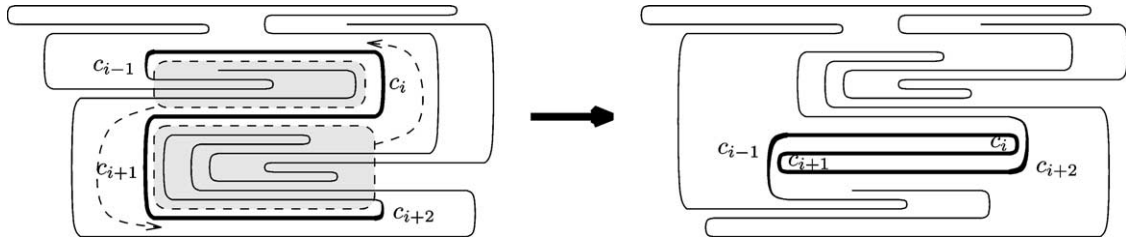
Fig. 11. Moving layers of paper out of the zig-zag formed by a crimp (c_i, c_{i+1}) , highlighted in bold.
