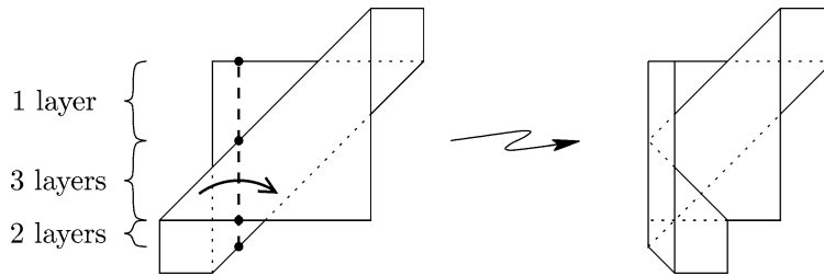
Fig. 6. Illustration of a simple fold in 2D (starting from Fig. 4, right), where we must specify the number of folded layers for each portion of the crease, because this number can vary along a single fold.
