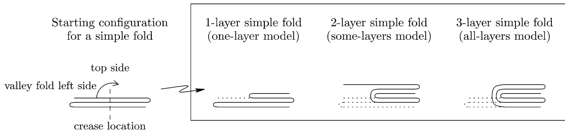
Fig. 5. Illustration of a simple fold in 1D, which is specified by a crease location, a notion of the “top side”, how many of the top layers are folded (here ranging from 1 to 3), whether the fold is mountain or valley, and whether the left or right side is folded.
