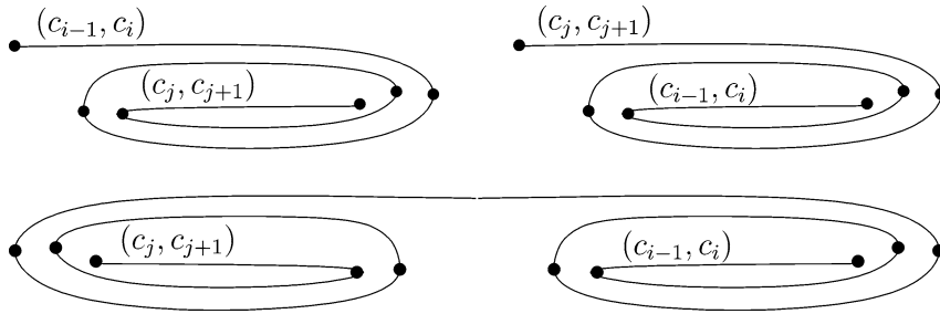
Fig. 9. The innermost edge of a spiral cannot be longer than the adjacent edge, in contrast to the outermost edge which can be arbitrarily long.
