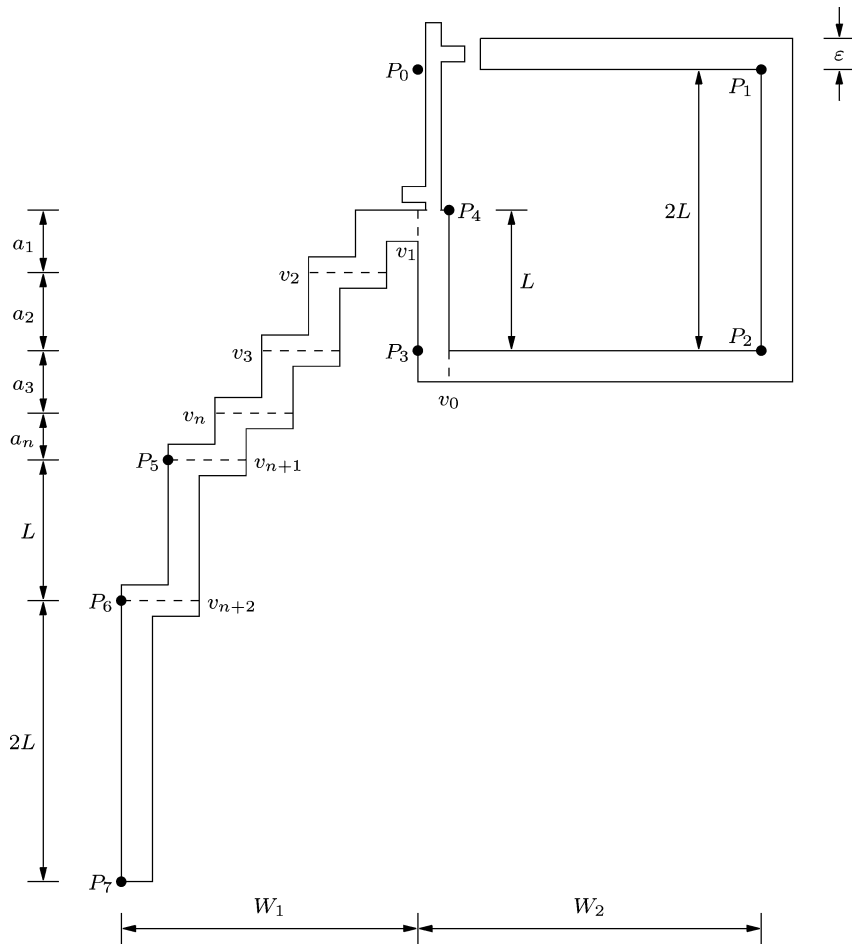
Fig. 17. Hardness reduction when no mountain-valley assignment is given.
