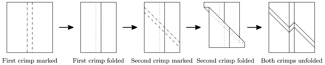
Fig. 19. Crimps intersecting at an angle other than 90 degrees cannot be folded out of order.
