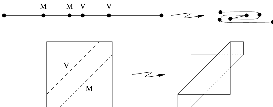
Fig. 4. Sample flat foldings in one and two dimensions. Mountains and valleys are denoted by M's and V's, respectively.
