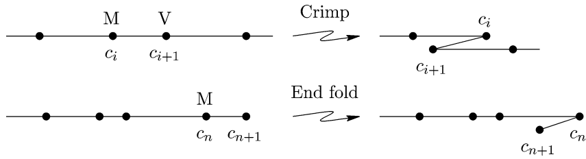
Fig. 8. The two local operations for one-dimensional one-layer folds.
