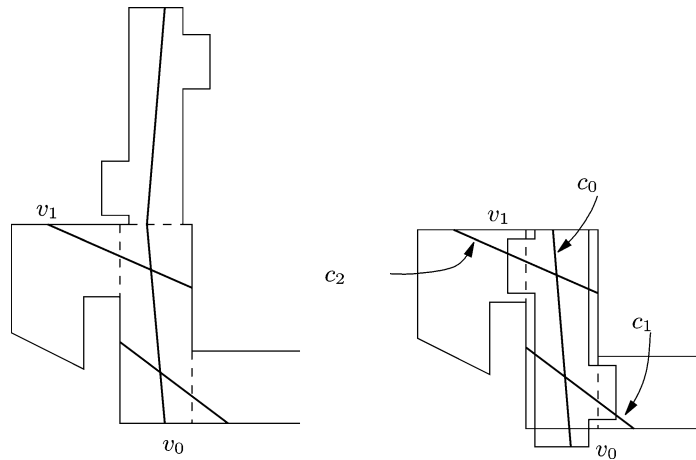
Fig. 18. Interesting part of construction for hardness reduction.
