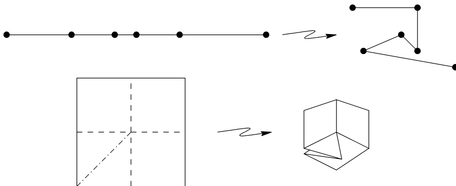
Fig. 3. Sample nonflat foldings in one and two dimensions.
