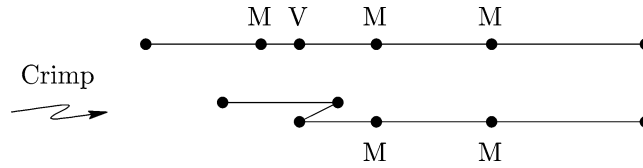
Fig. 10. A mingling mountain-valley pattern that when crimped is no longer mingling and hence not flat-foldable. Indeed, the original mountain-valley pattern is not flat-foldable.
