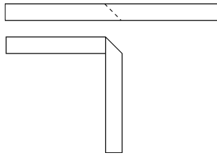
Fig. 15. Turning a strip.
