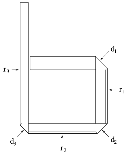
Fig. 16. Illustration of first few DR-folds used in construction.
