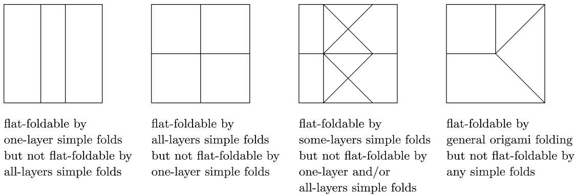
Fig. 7. Crease patterns illustrating the unique power of each model of simple folding, and the limitations compared to general flat folding.
