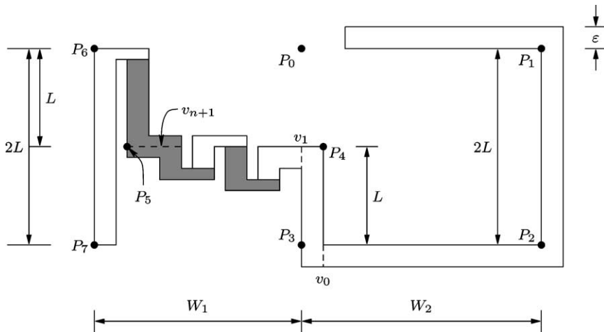
Fig. 14. Semi-folded staircase confined between y coordinates of P_1 and P_2 . The top side of the paper is drawn white and the other side is drawn gray.
