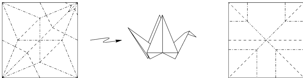
Fig. 1. Sample crease patterns. Left: the classic crane. Right: pattern of Hull [13], which cannot be folded flat, for any mountain-valley assignment.
