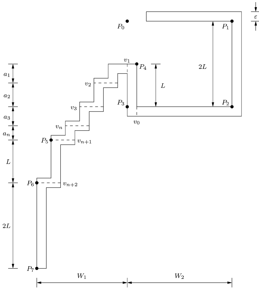
Fig. 13. Hardness reduction from PARTITION problem.
