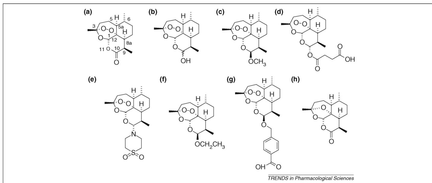
Figure 1. Chemical structures of artemisinins. Artemisinin ( a ) isolated in crystalline form in 1973 from Artemisia annua and derivatives dihydroartemisinin (DHA) ( b ), artemether ( c ), artesunate ( d ) and arteether ( f ) were first prepared by Chinese scientists in the 1970s [1]. Artemisone ( e ), representative of a new class of artemisinin known as amino-artemisinins, is curative in clinical trials at one-third the dose regimen of artesunate. It is characterized by low toxicity [56]. Artelinate ( g ) was prepared at the Walter Reed Army Institute of Research ( http://wrair-www.army.mil ), but was withdrawn because of toxicity concerns [112]. Deoxyartemisinin ( h ), lacking the peroxide bridge, is biologically inert.
