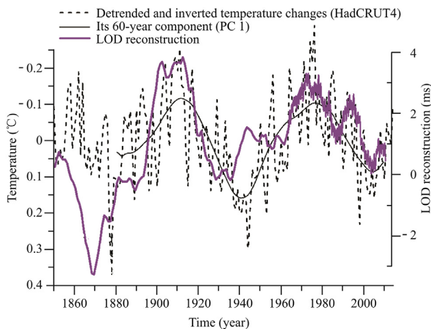
Fig. 3 – Long-term LOD compared with detrended and inverted temperature changes.
