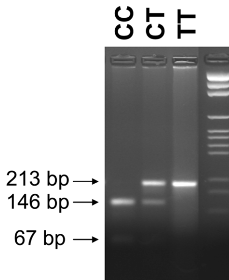
Figure 1 Restriction-enzyme analysis for the detection of the 932C→T (A282V) mutation. The 213-bp product is cleaved into two fragments, of 146 bp and 67 bp, in the presence of the wild-type sequence (CC). The mutated sequence is not cleaved (see lanes CT and TT).
