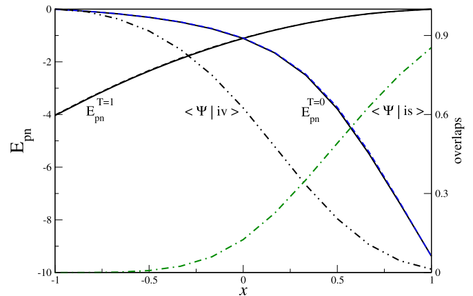
Fig. 1. proton–neutron pairing energies provided by the PQCM approach (full lines) and by exact diagonalization (dashed lines) together with the overlaps between the ground state (5) and the states (7) and (8). The parameter x on horizontal axis scales the strength of the interactions in the two pairing channels (see the text). The results correspond to 4 proton–neutron pairs moving in 10 equidistant levels and the pairing energies are given in units of levels spacing.
