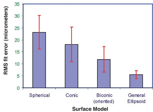
FIGURE 1 (RMS) fit errors obtained using four corneal models on 123 corneas: spherical, conic, biconic and general ellipsoid.
