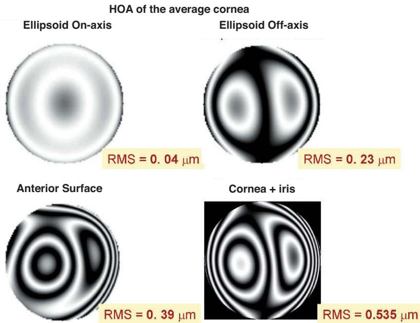
FIGURE 3 High-order aberrations of the mean cornea computed for a 6 mm pupil and a 550 nm wavelength.
