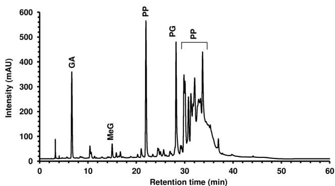
Fig. 1. HPLC-270 nm chromatogram of the hydroalcoholic extract from S. terbinthifolius leaves. GA, gallic acid. MeG, methyl gallate. PG, 1,2,3,4,6-pentagalloylglucose. PP, other gallic acid derivatives.
