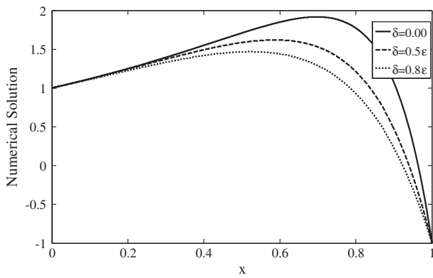
Figure 7 The numerical solution of example 4 with \epsilon = 0.1 .
