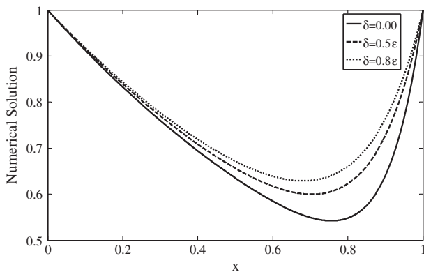
Figure 9 The numerical solution of example 5 with \epsilon = 0.1 .
