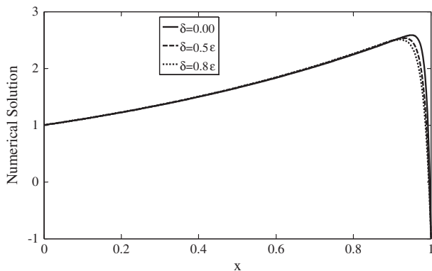
Figure 8 The numerical solution of example 4 with \epsilon = 0.01 .
