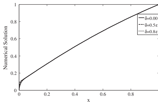
Figure 4 The numerical solution of example 2 with \epsilon = 0.01 .
