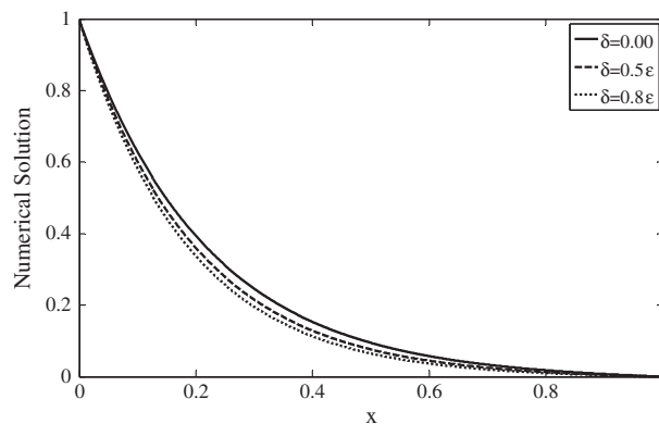
Figure 5 The numerical solution of example 3 with \epsilon = 0.1 .
