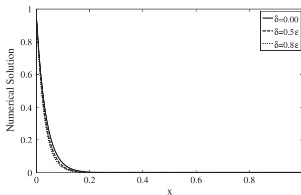
Figure 6 The numerical solution of example 3 with \epsilon = 0.01 .
