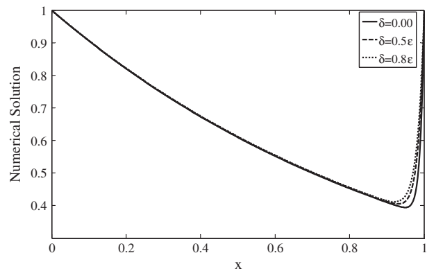
Figure 10 The numerical solution of example 5 with \epsilon = 0.01 .
