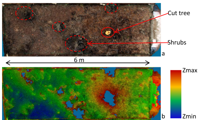
Fig. 6. Illustration of the effect of vegetation on soil surface microtopography showing a synoptic image of a 6 m \times 2 m erosion plot (a) and a digital elevation model of the relative elevation in the plot (b).
