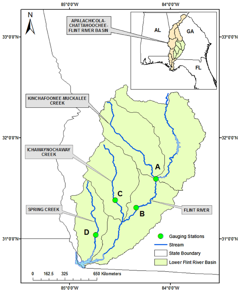
Fig. 1. The Lower Flint River (LFR) Basin showing the critical sub-watersheds. The stream flow gauging stations selected for this study are shown as green circles.
