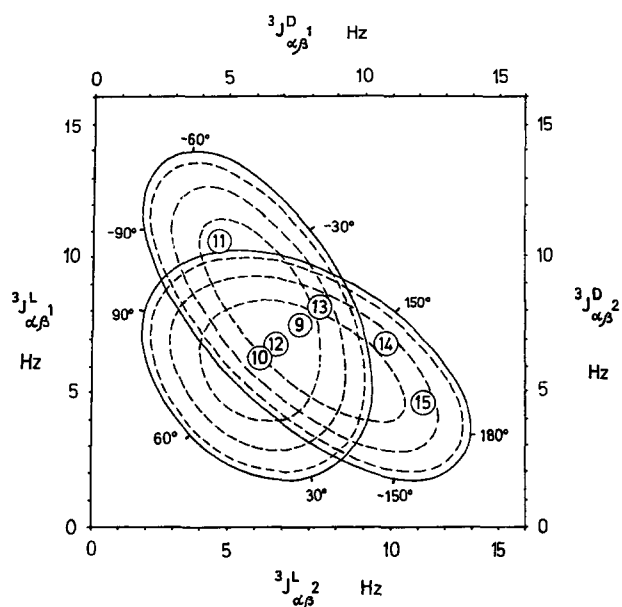
Fig. 1. Correlation diagram of coupling constant {}^3J_{\alpha\beta 1}^L - {}^3J_{\alpha\beta 2}^L . The solid line shows the relationship between SSC constants (fixed values of the torsion angle \chi^1 ). The dashed line shows the same relationship for side chain rapidly rotating around the \chi^1 -angle, characterized by Gaussian distribution with dispersion values of \sigma = 10^\circ, 20^\circ and 30^\circ . Experimental values of spin-spin coupling constants for L-Trp 11,15 and D-Leu 14 have been arranged in accordance with the most probably conformation (Fig. 2).
