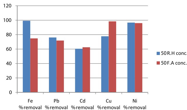
Fig. 7 Comparison between rice husk and fly ash removal efficiency at 50 mg/l adsorbent concentration.
