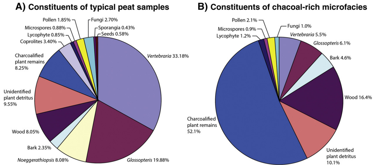
Fig. 3. Pie charts detailing the relative proportions of organic constituents in: A. typical permineralised peat of the Toploje Member chert taken from 4000 point counts at 200 µm increments from 20 thin Sections. B. charcoal-rich microfacies of the permineralised peat taken from 1000 point counts at 200 µm increments from 4 thin sections. Small quantities of pyrite crystals, and the silica matrix that occur in the Toploje Member chert were excluded from the counts.
