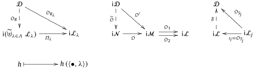
Fig. A.1. Product of i\mathcal{L}_\lambda 's is i(\tilde{\bigcup}_{\lambda \in \Lambda} \mathcal{L}_\lambda) (left), the equalizer i\mathcal{N} is constructed in a standard manner (middle), and coproduct of i\mathcal{L}_j 's is i\{\mathcal{L}_j \times \{j\} ; j \in J\} where j ranges over a finite set J (right).
