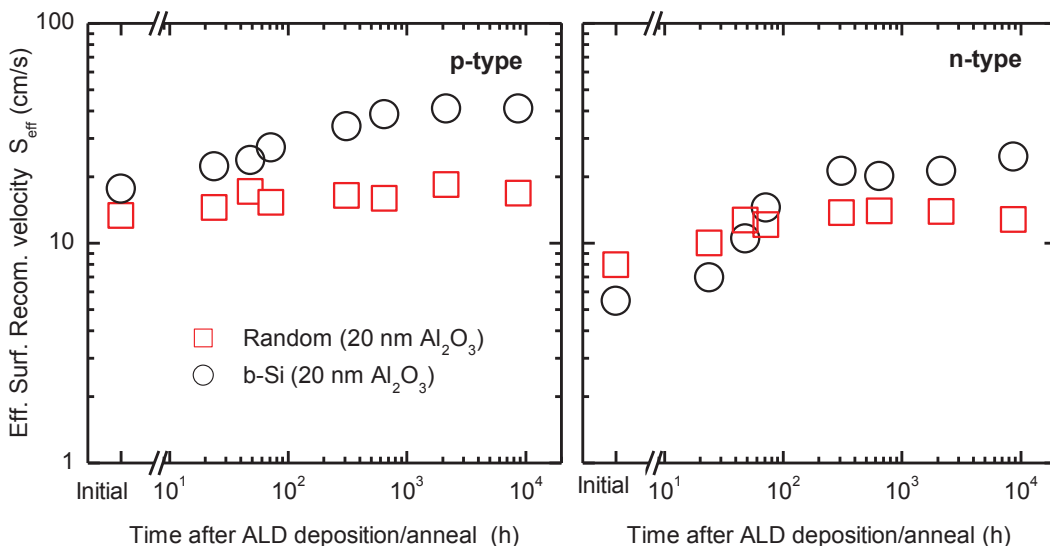
Fig. 3. S eff vs. time after ALD deposition and anneal for random (squares) and b-Si textured surfaces (circles) on a) p-type and b) n-type substrates. Samples were previously annealed at 400°C.
