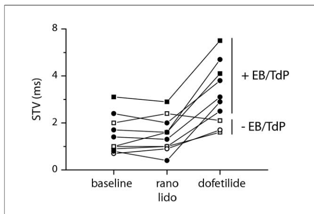
Figure 3 Relation Between STV and Ectopic Activity/TdP (EB/TdP)
