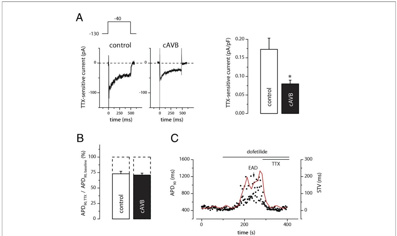
Figure 4 Late Na + Current Is Reduced in cAVB
