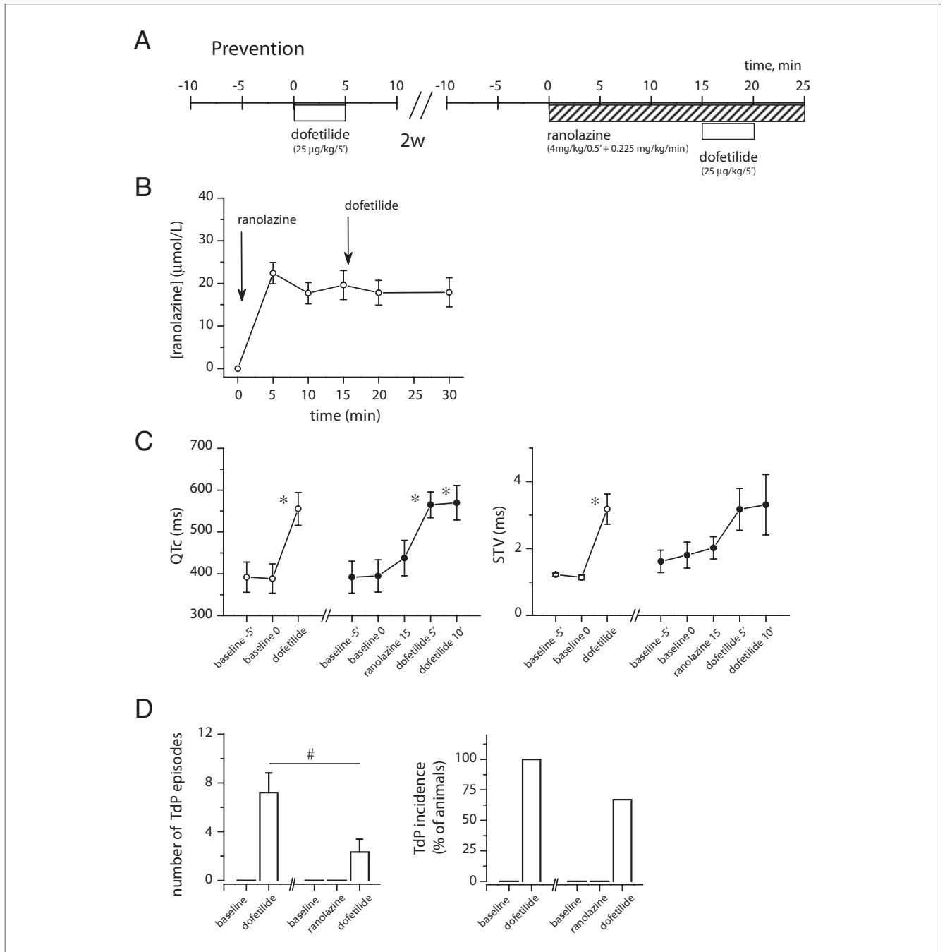
Figure 2 Prevention of TdP After Ranolazine Pre-Treatment
