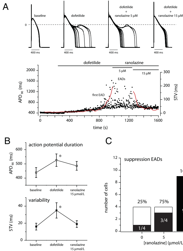
Figure 5 Ranolazine Suppression is Concentration-Dependent
