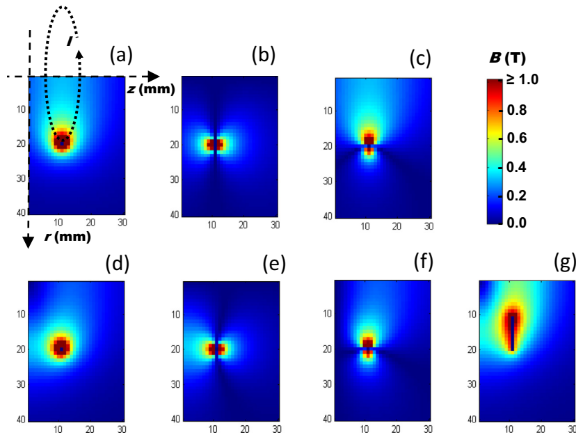
Fig. 3. Analytical field (Eq. (2)) of a current loop at 10 kA. (a) Total field amplitude, (b) radial field component, (c) axial field component. (d–f) Same current loop with mirror coil (placed at z = -10 and not visible here), representing an RF field over a metal plane at z = 0 . (d) Total field amplitude, (e) the radial field component is increased toward the metal plane, (f) the axial field component is nulled close to the metal plane. (g) 10 current loops at RF frequencies over a metal plane, modeling a situation similar to Fig. 2b: a pancake coil with certain R and f .
