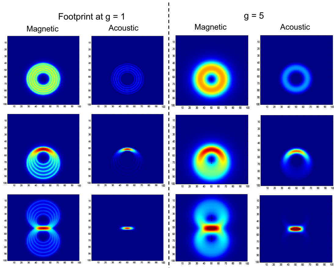
Fig. 6. Evolution of a butterfly coil from a circular, concentric pancake coil. All views in the target plane, at z = 0 mm. The magnetic and acoustic footprints from a normal pancake coil are shown in the first row. For g = 5 mm, the appearance of the magnetic and acoustic footprints becomes more diffuse, and a characteristic ring appears as the acoustic footprint. In the second row, the pancake has become excentric and the fields and acoustic effects are concentrated in the upper parts with high density. In the third row, an additional excentric pancake is superimposed in a way that that the concentrated parts are even more enhanced. A more spot-like footprint appears and the acoustic density is significantly increased, even over some distance ( g = 5 mm). The total energies for the three different arrangements at g = 5 mm are fairly equal.
