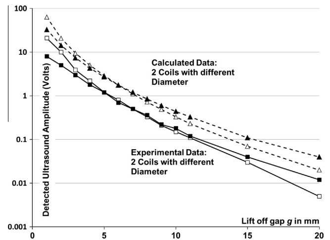
Fig. 4. Experimental ultrasound amplitudes (piezo raw signal in V) at 2 MHz over distance g from a small coil (white squares) and larger coil (black squares). Experimental data was copied from [9]. The calculation (Eq. (6), triangles) of coils with similar geometries results in quite similar behavior over distance. The calculated data are shifted upwards for a better representation, as there is not a measurable signal.
