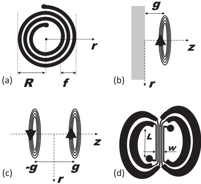
Fig. 2. (a) Flat spiral coil (“pancake coil”) with outer diameter R and active filling f . (b) The application is modeled as a number of concentric current circles placed over a metal plane at distance g . (c) Instead of a metal plane, a virtually identical field distribution in the right half space is obtained with a mirror coil with the same geometries and opposite current direction. (d) An alternative and more complex geometry (“butterfly coil”) consists of a concentrated (inner) part with high field densities and wider back wings (outside) with low field concentration.
