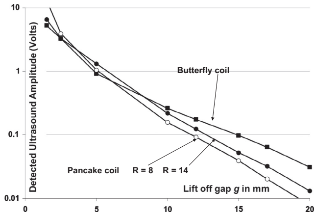
Fig. 7. Transmitted signal amplitudes from practical butterfly compared with practical pancake coils (28 mm diameter and 16 mm diameter, similar to Fig. 4); target area is 30 mm-diameter aluminum. At greater distances g , the butterfly is clearly superior and delivers about five times the signal power (=squared amplitude) at g = 20 mm.
