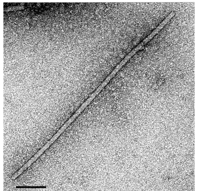
Fig. 2. Electron micrograph of a particle of AFV1 with an envelope removed by 0.1% Triton X-100, negatively stained with 3% uranyl acetate. Bar, 100 nm.
