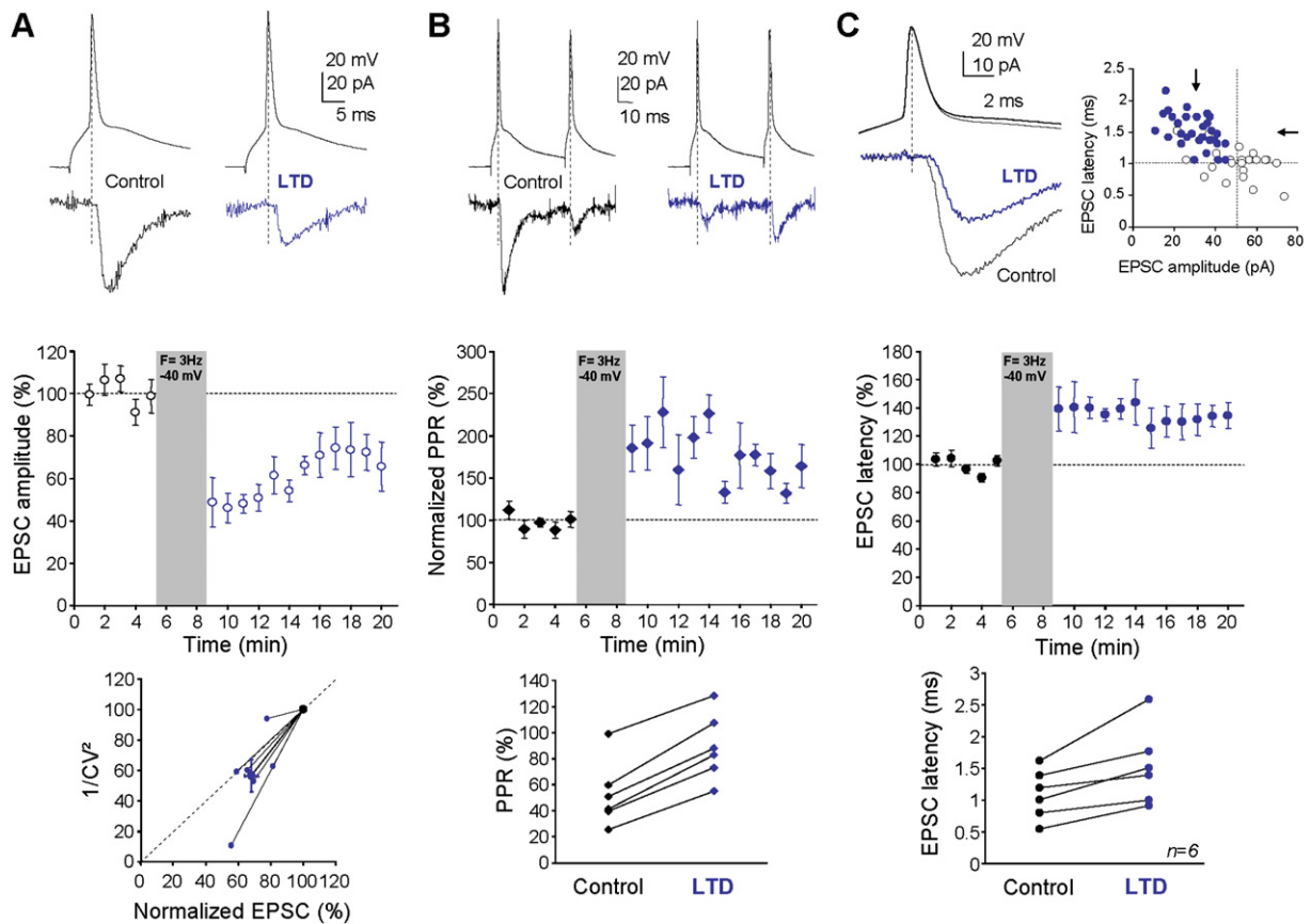
Figure 5. Change in Latency Associated with Presynaptic LTD at L5-L5 Synapse
