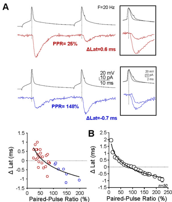
Figure 4. Synaptic Latency during Short-Term Synaptic Plasticity at L5-L5 Connections Tested with Pairs of Presynaptic APs (ISI = 50 ms)
