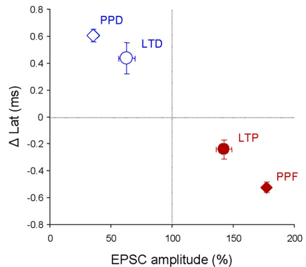
Figure 8. Activity-Dependent Changes in Latency at L5-L5 Connection
