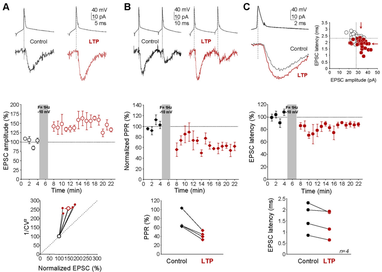
Figure 6. Change in Latency Associated with Presynaptic LTP at L5-L5 Synapse
