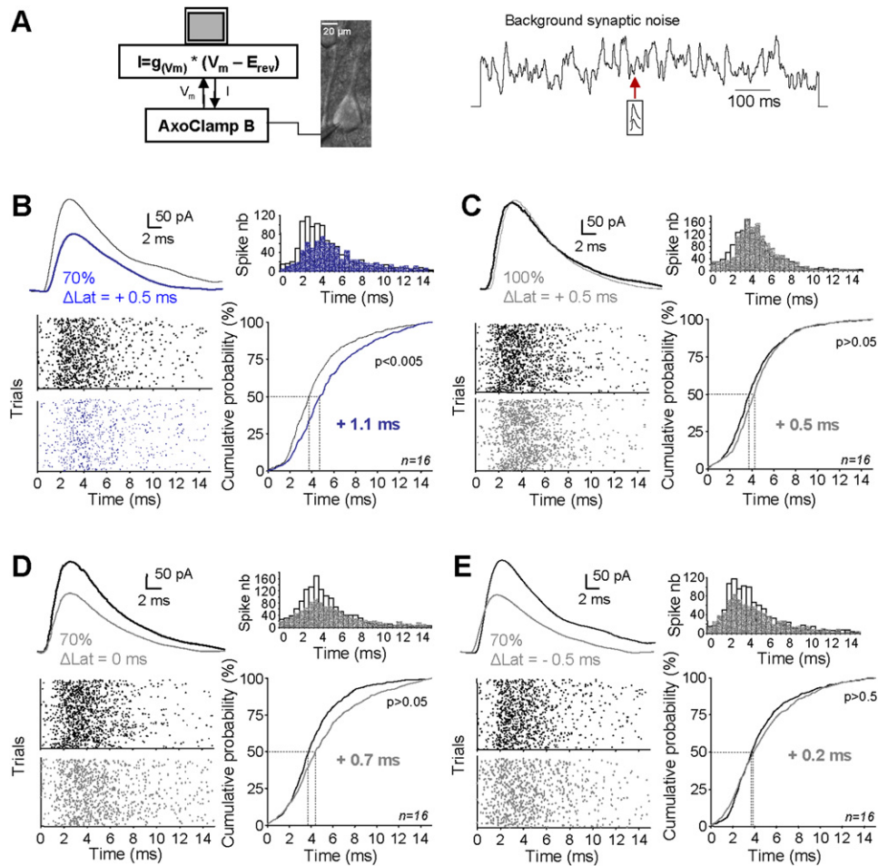
Figure 7. Effect of EPSP Modifications on Input/Output Function in L5 Pyramidal Neurons
