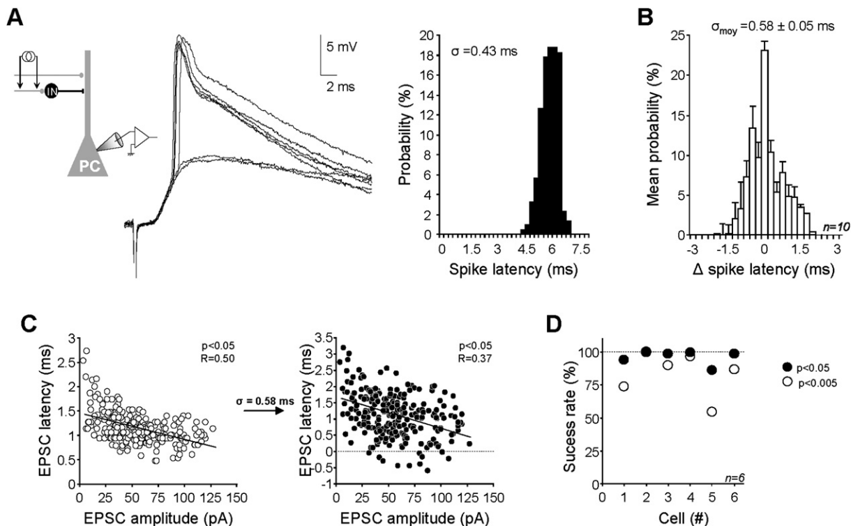
Figure 2. The Jitter of the Presynaptic Spike Does Not Suppress Pr -Dependent Latency Correlation in L5 Pyramidal Cells
