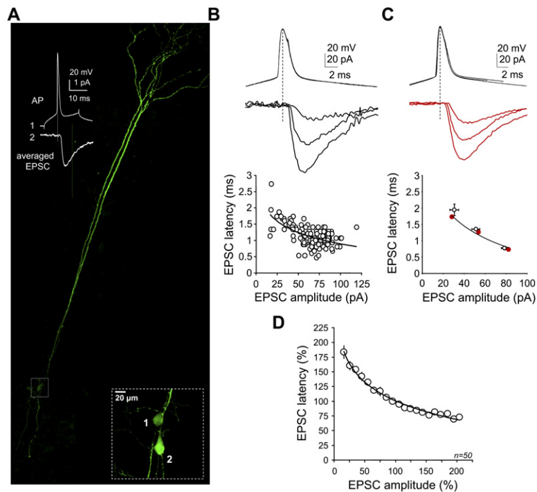
Figure 1. Amplitude-Dependent Latency Variation at L5-L5 Synapse
