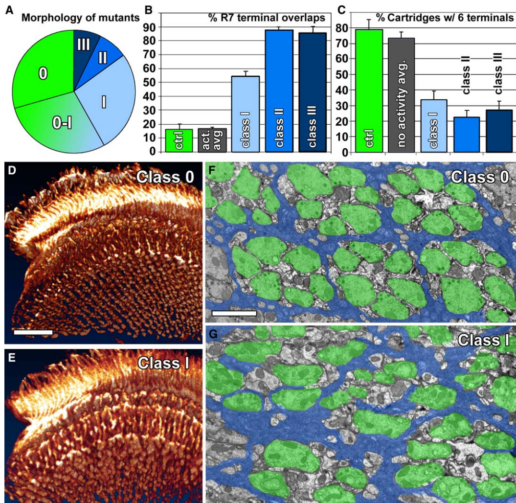
Figure 2. Forward Genetics: Novel Mutants Isolated in a Screen for Defects in Synapse Formation and Function Display Several Classes of Photoreceptor Projection Defects
