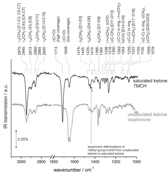
Fig. 7. IR spectra of 1.5 ML of TMCH (black) and isophorone (gray) adsorbed at 120 K on Pd(111) in the frequency range 3100–2700 \text{cm}^{-1} (C–H stretching), 1800–1600 \text{cm}^{-1} (C=C and C=O stretching), and 1500–1000 \text{cm}^{-1} (C–H and C–C deformation and C–C stretching).
