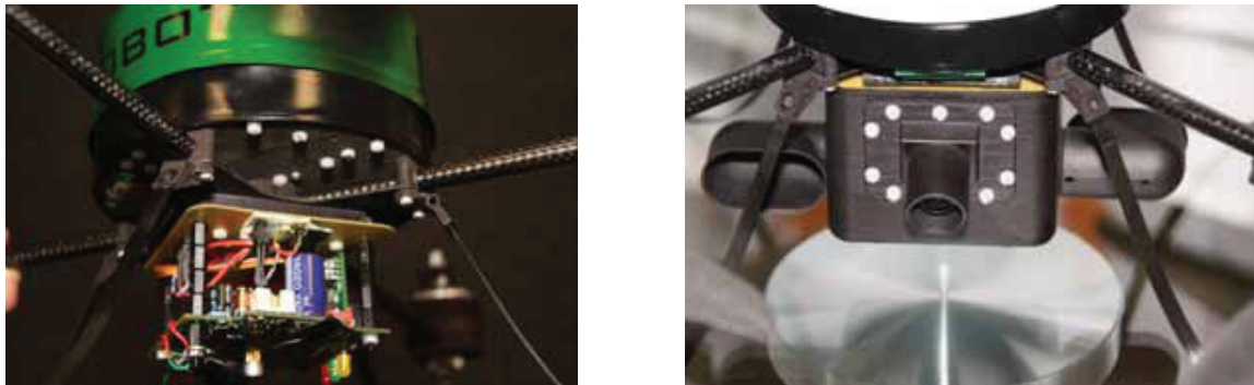
Fig. 6. AirRobot UAV with gas sensors and a camera.
