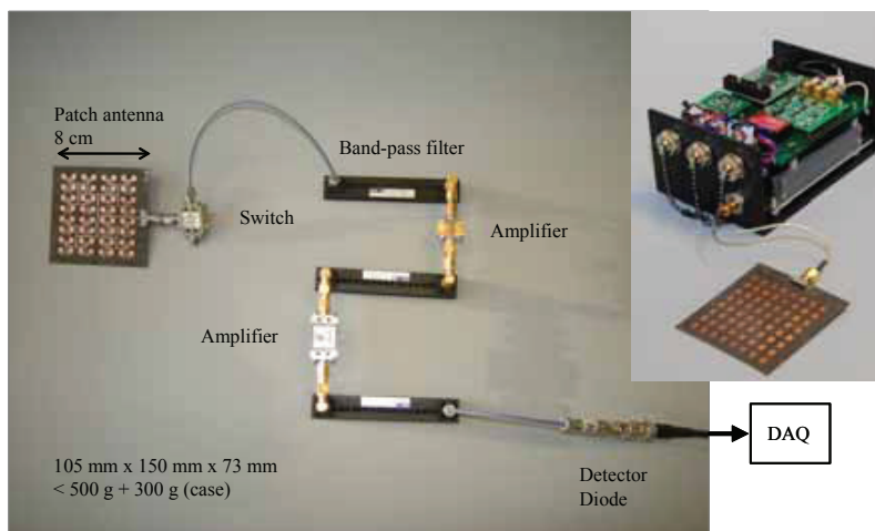
Fig. 14. Image of the 22.3 GHz radiometer.
