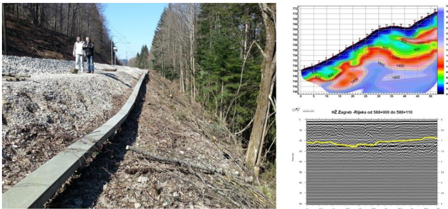
Fig. 8. Unstable embankment at km 588+000 do km 588+110, railway M 202 in Croatia, with belonging refraction profile and GPR profiles recorder during the assessment stage.
