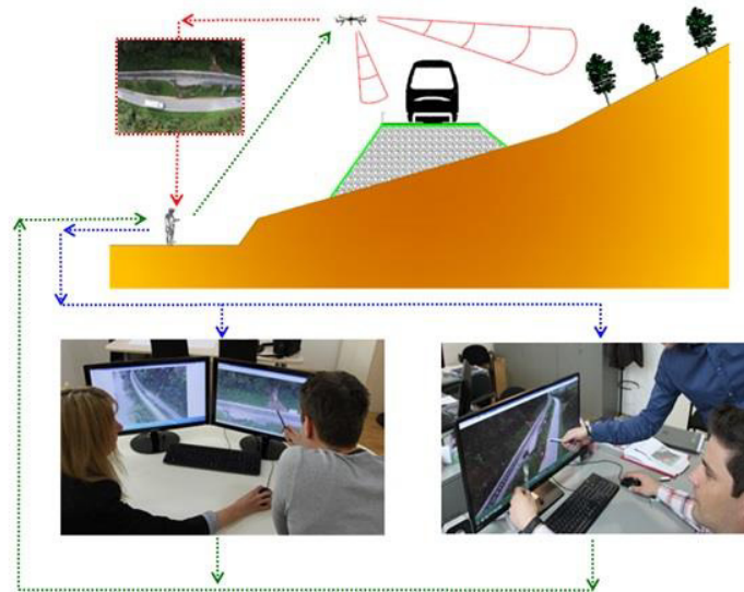
Fig. 4. Interactive procedure of visual assessment using UAV.
