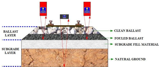
Fig. 5. Typical configuration of the GPR testing applied on the railway infrastructure (Bekic, 2015).
