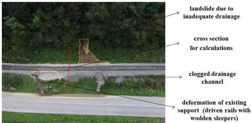
Fig. 2. Typical problem of embankment instability – image recorded with UAV, as a part of the repair project on railway track in Croatia.
