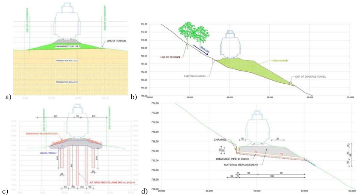
Fig. 3. Examples of typical problems a) cross section of the embankment with soft soil, and b) instability problem due to the lack of drainage system, c) remediation measure for the case a); d) remediation measure for the case b).
