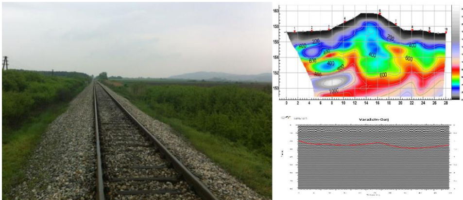
Fig. 7. Unstable embankment at km 132+200 till km 133+000, railway track R202 in Croatia, with belonging refraction profile and GPR profiles recorder during the assessment stage.
